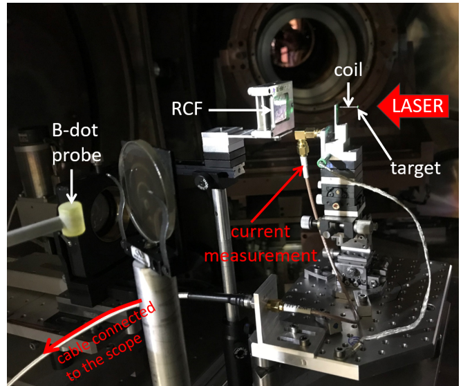
FIG. 1. Experimental set-up.
