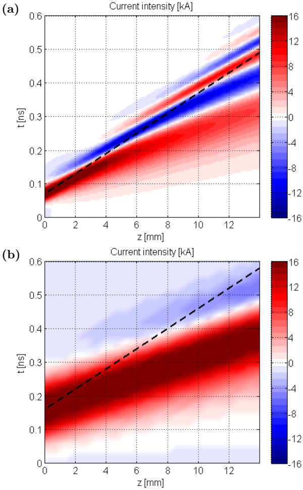
FIG. 14. Model of the current pulse propagation along the helical coil. Comparison for an initially short ( \tau_e = 15 ps) (a) and long ( \tau_e = 60 ps) (b) pulse emission. The helical coil has a radius a = 0.5 mm and a pitch p = 0.35 mm. Figures obtained from the numerical resolution of Eq. (6).
