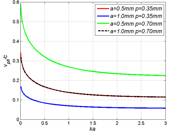
Velocity ratio v_{ph}/c function of the wave number k , radius a and pitch p of the helix
