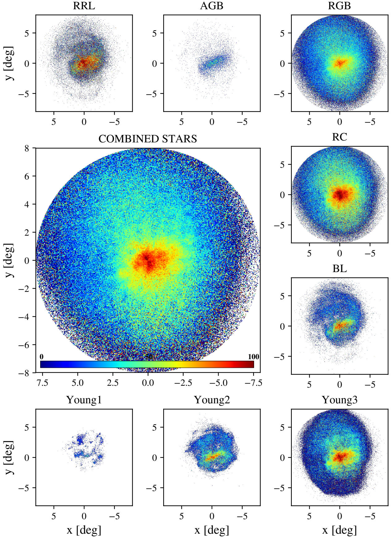
Fig. B.4. Radial velocity dispersion maps \sigma_R of the LMC for the combined sample ( main panel ) and the various evolutionary phases. The linear velocity scale shown by the colour bar in the main panel is the same in all subpanels and has been chosen to highlight velocity patterns better.
