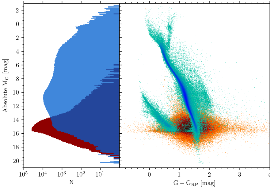
Fig. 2. Left panel: distribution of absolute G magnitudes for the full Gaia EDR3 \varpi \geq 8 mas sample. The blue distribution is for selected sources and the red one for rejected sources using a bin size of \sigma_{M_G} = 0.1 mag. The slight bump in the distribution of selected sources at M_G = 15 mag that coincides with the maximum of the rejected sources is probably indicative of contamination. Right panel: CAMD diagram for the full sample. The blue points are good solutions and the red poor ones. The strip of source with nominally good solutions connecting the main and white dwarf sequence at M_G \sim 15 is unexpected and due to contamination of the GCNS by faint objects at distances of 80–120 pc, as discussed in Sect. 4.5.
