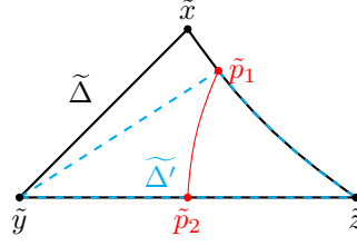
■ Figure 9 The two triangles \tilde{\Delta} and \tilde{\Delta}' in the proof of Proposition 16.
