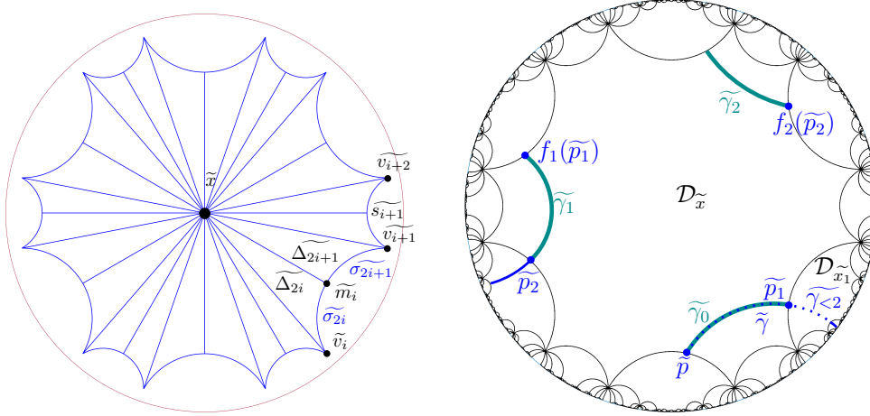
(a) The triangles partitioning \mathcal{D}_x (illustration for the special case of TMPS). (b) Representation of a geodesic path \tilde{\gamma} as a sequence of segments in \mathcal{D}_x . The path \tilde{\gamma}_{<2} is also shown as a dashed part of \tilde{\gamma} .
