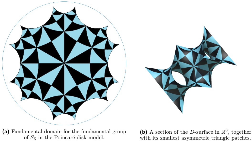
■ Figure 1 The covering of the diamond TPMS by \mathbb{H}^2 .
