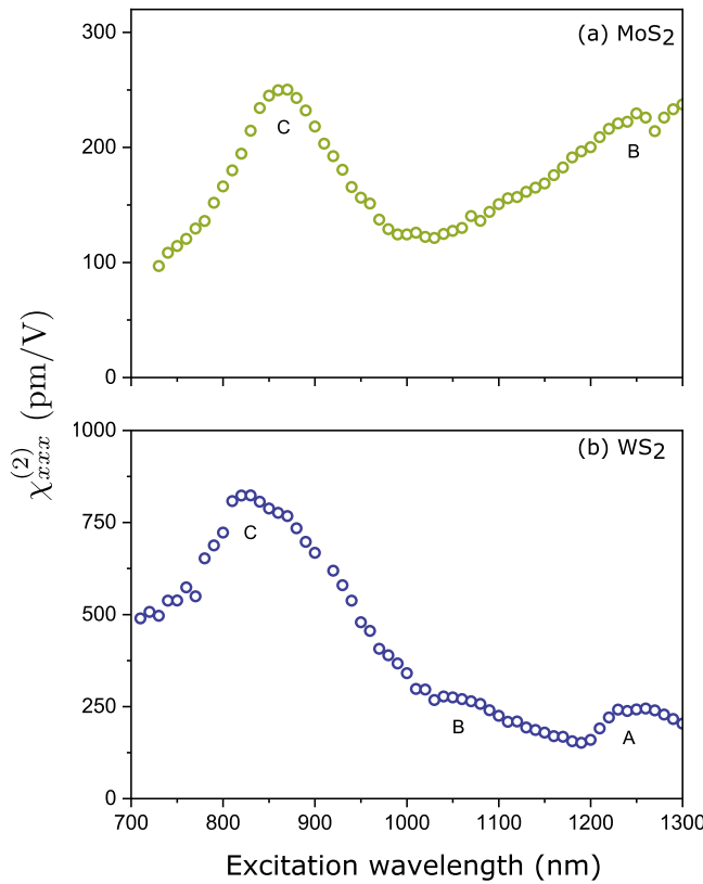
FIG. 4. Absolute nonlinear susceptibility \chi_{xxx}^{(2)} of (a) MoS 2 and (b) WS 2 (sample w2; see Table I).
