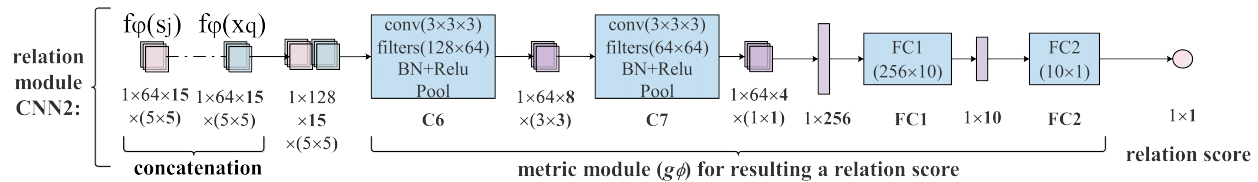
Figure 5. Architecture of the relation model to measure the similarity between deep features f_\varphi(s_j) and f_\varphi(x_q) .
