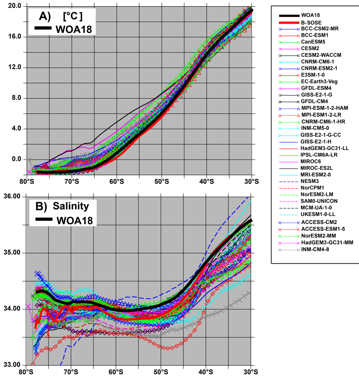
FIG. 5. The zonally averaged and time-averaged near-surface (a) potential temperature ( ^{\circ}\text{C} ; 0–100 m average), and (b) salinity (0–100-m average). The CMIP6 model output are time-averaged from January 1986 to December 2005. The January 2013 – December 2018 time period is averaged for the B-SOSE Iteration 133 solution. The WOA18 values are computed from the average of the 1985–94 and 1995–2004 decadal climatologies.
