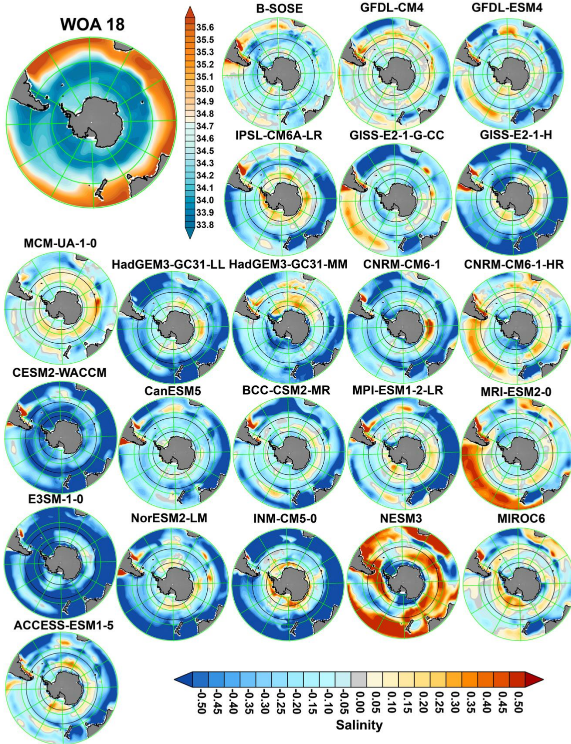
FIG. 6b. As in 6a, but for salinity in the upper ocean (0 – 100 m average). Positive (from yellow to red) values indicate the model is more saline than observed. Negative (blue) values indicate the model is fresher than observed. Additional models are shown in the Supplemental Material.
