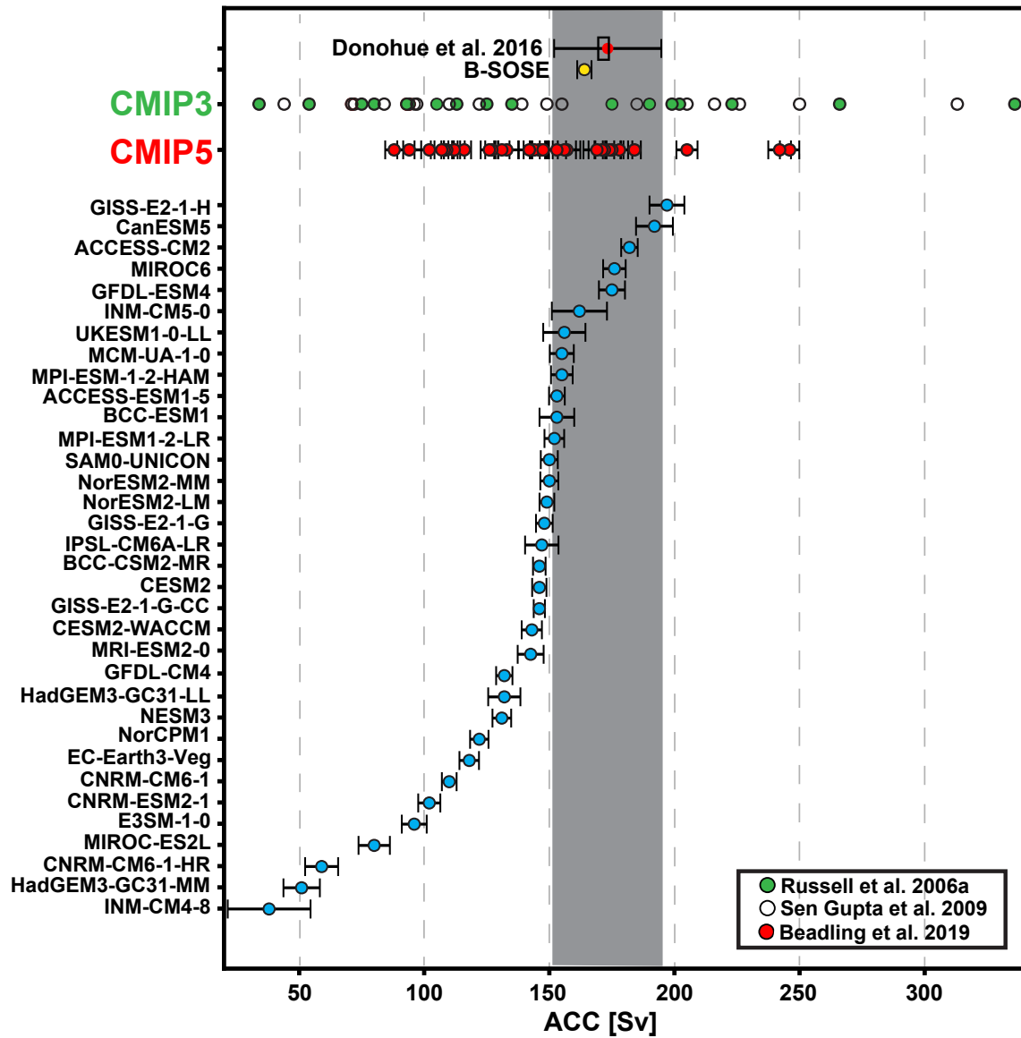
FIG. 1. Volume transport of the ACC through the Drake Passage (Sv) as observed from the cDrake experiment (Donohue et al. 2016) and as simulated across multiple generations of climate models. Gray shading corresponds to the observational uncertainty ( 2\sigma ) of the ACC transport reported in Donohue et al. (2016). The B-SOSE transport is computed from the Iteration 133 solution at 1/6^{\text{th}} degree resolution over the January 2013 to December 2018 time period. The CMIP6 model transports are calculated as the January 1986 to December 2005 time-averaged net transport through the Drake Passage. The CMIP5 values are taken from Beadling et al.
