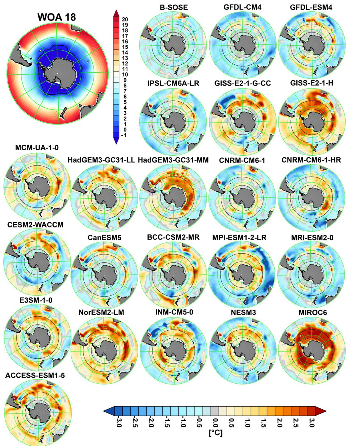
FIG. 6a. Upper ocean potential temperature (°C) (0 -100 m average) in the Southern Ocean from the WOA18 climatological mean (large panel at top left; computed from the average of the
