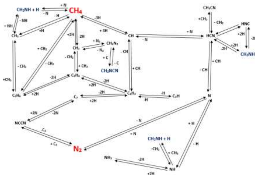
Fig. 4. Reaction pathways for formation of hydrocarbons and C-N compounds, including methylenimine and cyanomethanimine.
