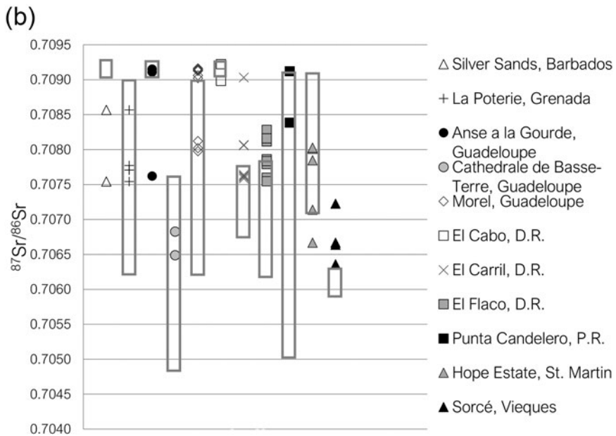
Figure 2. (a) Bivariate plot of dog \delta^{15}\text{N} and \delta^{13}\text{C} values from El Flaco and El Carril, Dominican Republic; Morel and Cathédrale de Basse-Terre, Guadeloupe; and Hope Estate, Saint-Martin (Shev 2018); (b) chart showing the estimated bioavailable ^{87}\text{Sr}/^{86}\text{Sr} local ranges (represented by boxes) of each site/island and whether each sample fits into or outside these ranges.
