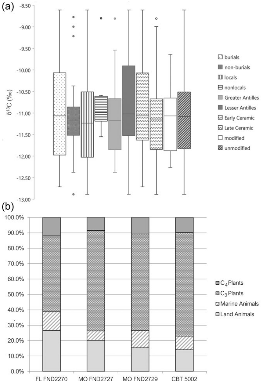
Figure 3. (a) Box plot showing median \delta^{13}C_{en} values (horizontal line), inner quartiles (box), value ranges (whiskers), and outliers (dots) for all comparative parameters; (b) FRUITS dietary mixing model results for El Flaco (FND 2270), Morel (FND 2727 and FND2729), and Cathédrale de Basse-Terre (CBT5002).
