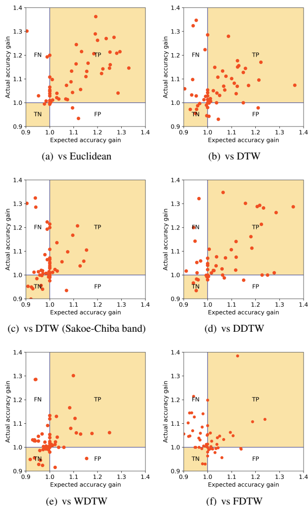
FIGURE 6. Texas sharpshooter plot of TAOT versus the other six competing methods respectively.
