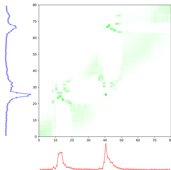
FIGURE 8. A fuzzy warping path generated by TAOT.
