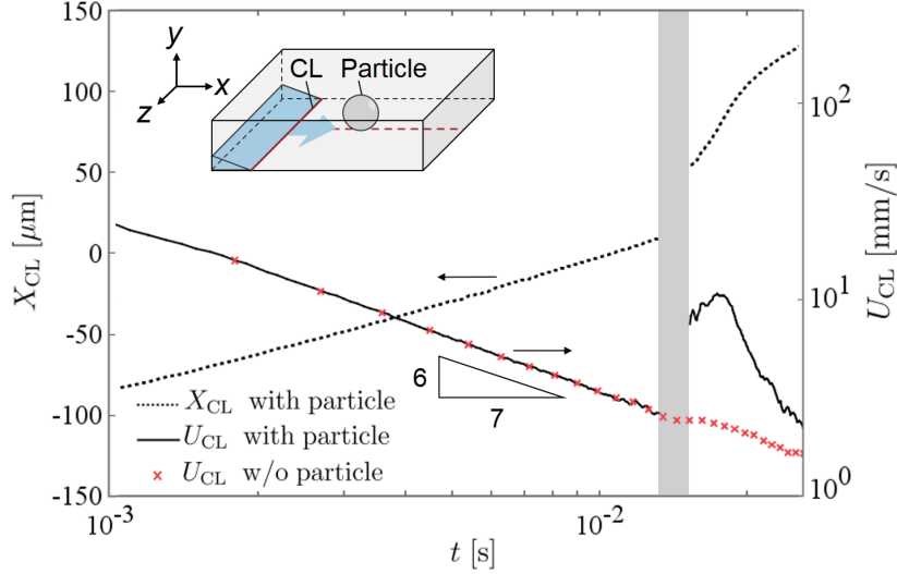
Figure 5: Temporal variations of the CL position X_{\text{CL}} and velocity U_{\text{CL}} on substrates. The CL position is derived on the line parallel to the x direction passing under the particle foot on the substrate as illustrated in inset. Note that the CL position is not well defined in the gray area, in which the CL is traveling around the particle foot.
