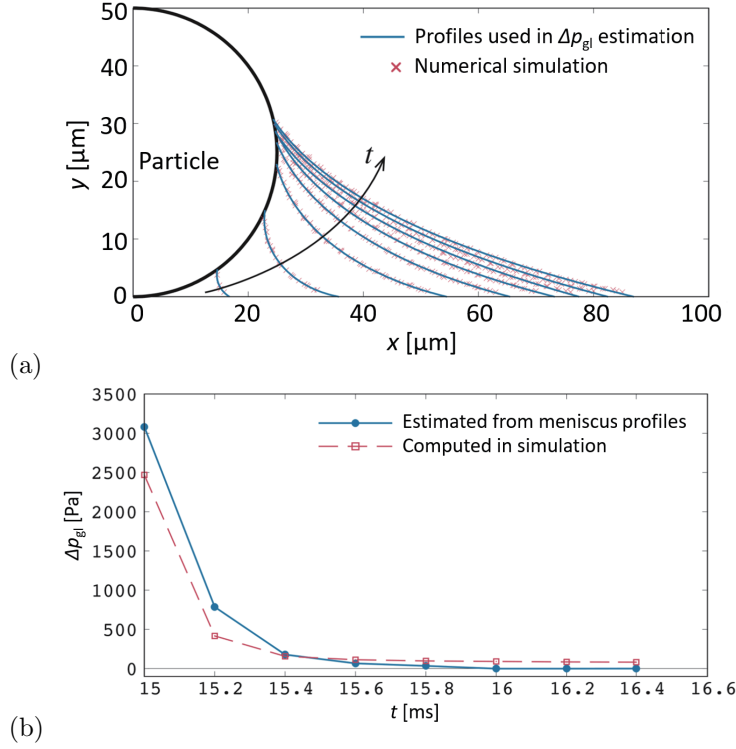
Figure A.1: (a) Profiles of a downstream side of meniscus developing around a spherical particle at t = 15, 15.2, 15.4, 15.6, 15.8, 16, 16.2, and 16.4 ms. Profiles determined in a numerical simulation and theoretical ones are compared. The latter profiles are used to estimate Laplace pressure \Delta p_{\text{gl}} . (b) Temporal variation of the pressure difference \Delta p_{\text{gl}} at gas-liquid interface of downstream side of meniscus by estimation based on Laplace pressure and simulation.
