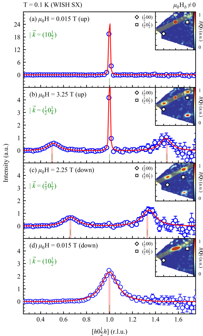
FIG. 2. ( T = 0.1 K) scans along [h0\frac{h}{2}] from WISH. On increasing the field momentum broadened \vec{k} = (\frac{1}{2}0\frac{1}{4}) [panel (b)] peaks draw intensity from \bar{Q} = (10\frac{1}{2}) . On decreasing the field from saturation, these are replaced by momentum broadened peaks at \vec{k} = (\frac{2}{3}0\frac{1}{3}) . At low fields [panel (d)], the zero-field structure is characterized by \vec{k} = (10\frac{1}{2}) but spatially short ranged. The solid curves are fits described in the main text, and red bars are the resolution.
