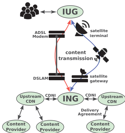
Fig. 1: Hybrid architecture
