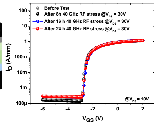
Figure 8. Transfer characteristics before and after 8, 16 and 24 hours of 40 GHz RF stress at V_{DS} = 30 V at room temperature.
