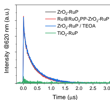
Figure 4. Time-resolved luminescence decays measured at 620 nm by laser flash photolysis (excitation at 532 nm) of thin films in \text{N}_2 -purged aqueous solutions: \text{ZrO}_2\text{-RuP} in 0.1 M \text{Na}_2\text{SO}_4 at pH 7 (black trace), \text{Ru@RuO}_2\text{PP-ZrO}_2\text{-RuP} in 0.1 M \text{Na}_2\text{SO}_4 at pH 7 (red trace), \text{ZrO}_2\text{-RuP} in
