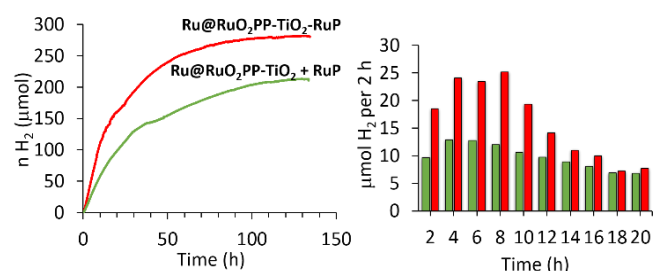
Figure 3. Photocatalytic hydrogen evolution profile (left) and hydrogen evolution rate per 2h (right) for \text{Ru@RuO}_2\text{PP-TiO}_2 (4 mg) + [\text{RuP}] = 0.1 mM (green) and \text{Ru@RuO}_2\text{PP-TiO}_2\text{-RuP} (red) under visible-light irradiation in a 4 mL TEOA 0.2 M aqueous solution at pH 7.
