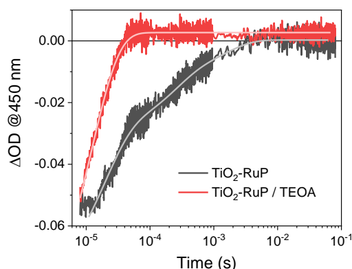
Figure 5. Transient absorption kinetics at 450 nm measured by laser flash photolysis (excitation at 532 nm) of TiO 2 -RuP in N 2 -purged aqueous solutions containing 0.1 M Na 2 SO 4 at pH 7 (black trace) and 0.2 M TEOA at pH 7 (red trace).
