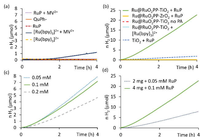
Figure 2. Photocatalytic hydrogen evolution in 4 mL of a 0.2 M TEOA aqueous solution of: (a) Unsupported Ru@RuO 2 PP with different PA (0.1 mM); (b) Supported Ru@RuO 2 PP-TiO 2 (M = Ti, Zr) with 0.1 mM [Ru(bpy) 3 ] 2+ , 0.1 mM RuP, no PA, and the corresponding TiO 2 -RuP blank; (c) Optimization of RuP PA concentration in the photocatalytic hydrogen evolution of Ru@RuO 2 PP-TiO 2 (2 mg); (d) Study of the Ru@RuO 2 PP-TiO 2 concentration at the optimized Ru@RuO 2 PP-TiO 2 / RuP ratio.
