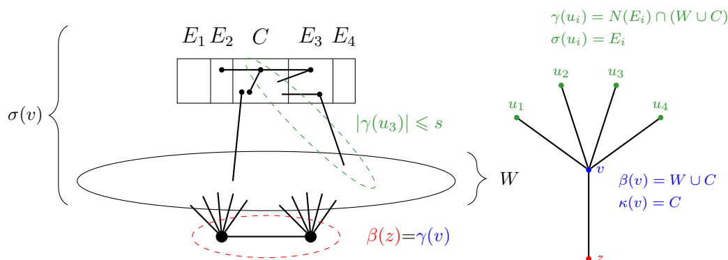
Figure 2: A schematic illustration of the construction of the tree decomposition in the proof of Lemma 21, in the case where |W| > (\Delta - 1)^{b-1} s and v is thus a branching vertex.
