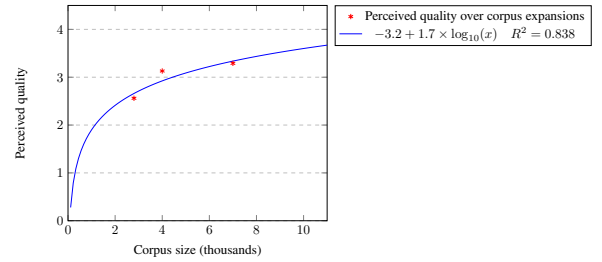
Figure 2. Subjective quality vs. corpus size.
