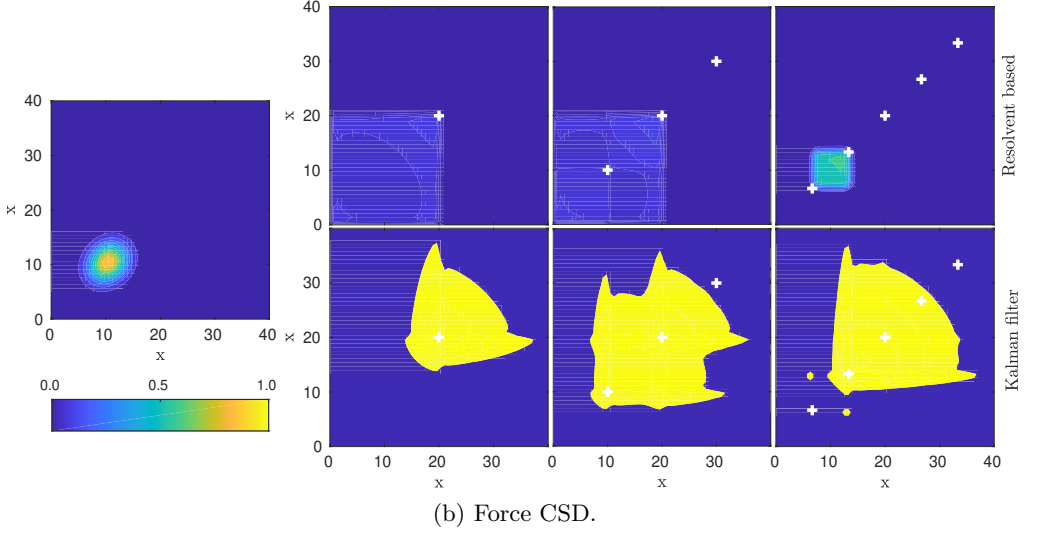
Figure 11: Same as figure 8 for frequency-dependent CSDs. Estimation for \omega = 3 .
