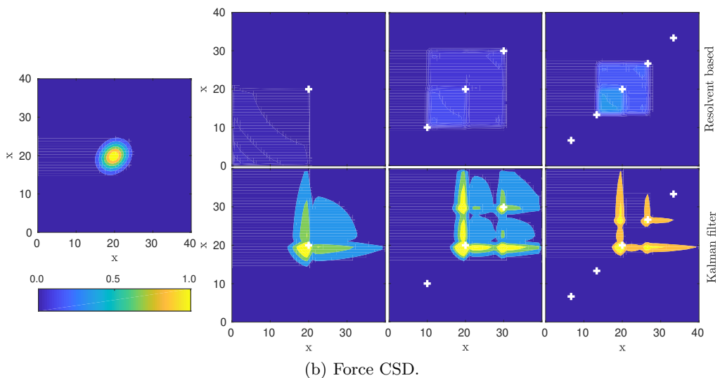
Figure 10: Same as figure 8 for frequency-dependent CSDs. Estimation for \omega = 1 .
