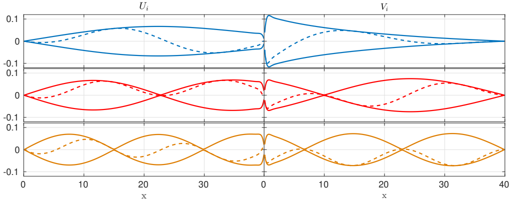
Figure 4: Ginzburg-Landau response (left) and force (right) modes. From top to bottom are the optimal and first two suboptimal modes. Solid lines correspond to the amplitude envelope and dashed lines show the real part.
