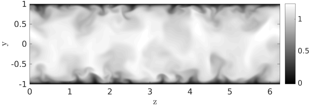
Figure 25: Snapshot of the streamwise velocity component of the turbulent channel flow.
