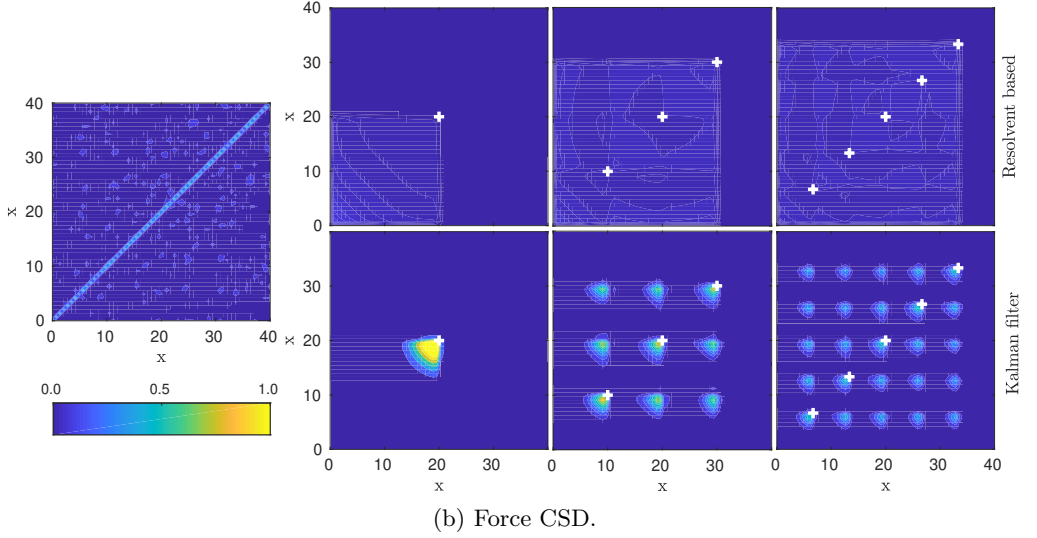
Figure 9: Same as figure 8 for CSD at \omega = 1 .
