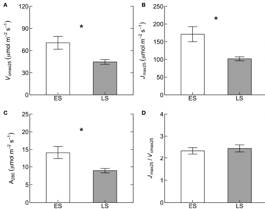
FIGURE 1 | Photosynthetic traits at 25°C. Maximum rates of (A) Rubisco carboxylation capacity ( V_{c\max 25} , \mu\text{mol m}^{-2} \text{s}^{-1} ) and (B) electron transport ( J_{\max 25} , \mu\text{mol m}^{-2} \text{s}^{-1} ), (C) photosynthetic rates at a constant intercellular \text{CO}_2 concentration (C) of 280 ppm ( A_{280} , \mu\text{mol m}^{-2} \text{s}^{-1} ), and (D) the ratio of J_{\max 25} to V_{c\max 25} ( J_{\max 25}/V_{c\max 25} ) in early-successional (ES, white) versus late-successional (LS, gray) tree species in Nyungwe forest. The asterisks (in A–C ) indicate statistical significance ( p < 0.05 ). Error bars represent SE with n = 5\text{--}7 species per successional group and 7–15 trees per species.
