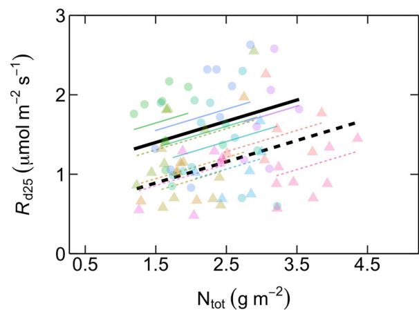
FIGURE 5 | Relationship between dark respiration at 25^{\circ}\text{C} ( R_{\text{d}25} , \mu\text{mol m}^{-2} \text{ s}^{-1} ) as a function of area-based total leaf nitrogen content ( N_{\text{tot}} , \text{g m}^{-2} ) in early-successional (ES) and late-successional (LS) tree species in Nyungwe forest. Different symbol colors represent each of the 12 studied species, and symbol shapes represent successional groups (ES = circle; LS = triangle). Black solid (ES: R_{\text{d}25} = 0.27 N_{\text{tot}} + 0.99 ) and dashed (LS: R_{\text{d}25} = 0.27 N_{\text{tot}} + 0.5 ) lines are overall regression lines for ES (solid) and LS (dashed) groups, respectively, but with common slopes since these did not significantly differ. Colored lines represent regression lines for each species belonging to ES (solid) and LS (dashed) groups. n = 5\text{--}7 species per successional group and 7–15 trees per species.
