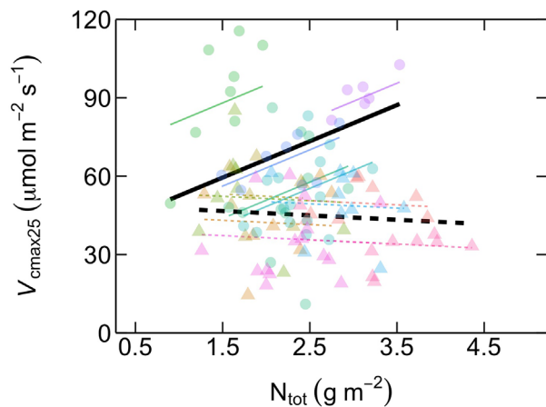
FIGURE 4 | Relationship between maximum rates of Rubisco carboxylation capacity at 25^{\circ}\text{C} ( V_{\text{cmax}25} , \mu\text{mol m}^{-2} \text{ s}^{-1} ) as a function of area-based total leaf nitrogen content ( N_{\text{tot}} , \text{g m}^{-2} ) in early-successional (ES) and late-successional (LS) tree species in Nyungwe forest. Different symbol colors represent each of the 12 studied species, and symbol shapes represent successional groups (ES = circle; LS = triangle). Black solid (ES: V_{\text{cmax}25} = 13.9 N_{\text{tot}} + 38.6 ) and dashed (LS: V_{\text{cmax}25} = -1.6 N_{\text{tot}} + 49.1 ) lines are overall regression lines for ES and LS groups, respectively. Colored lines represent regression lines for each species belonging to ES (solid) and LS (dashed) groups, respectively, but with common successional group-specific slopes. n = 5\text{--}7 species per successional group and 7–15 trees per species.
