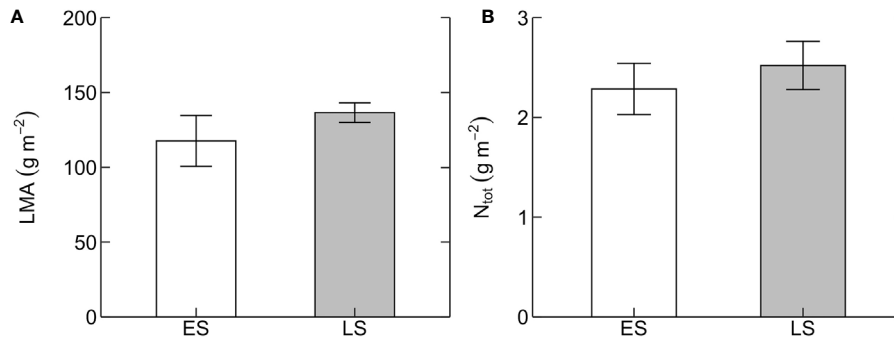
FIGURE 3 | Leaf structural and chemical traits. (A) Leaf mass per unit leaf area (LMA, \text{g m}^{-2} ) and (B) area-based total leaf nitrogen content ( N_{\text{tot}} , \text{g m}^{-2} ) in early-successional (ES, white) and late-successional (LS, gray) tree species in Nyungwe forest. Error bars represent SE with n = 5\text{--}7 species per successional group and 7–15 trees per species.
