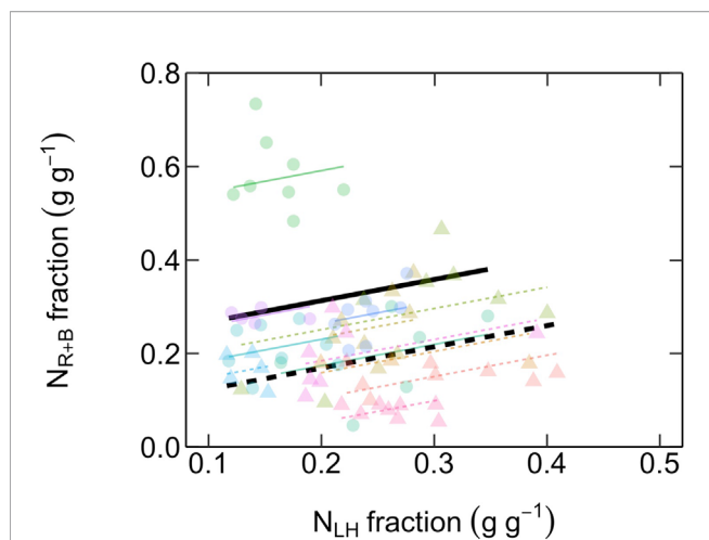
FIGURE 6 | Relationship between fractional investments of total leaf N content into compounds maximizing photosynthetic capacity ( N_{R+B} , g\ g^{-1} ) and compounds maximizing photosynthetic light-harvesting ( N_{LH} , g\ g^{-1} ). Different symbol colors represent each of the 12 studied species, and symbol shapes represent successional groups (ES = circle; LS = triangle). Black solid and dashed lines are overall regression lines for ES ( N_{R+B} = 0.45 N_{LH} + 0.22 ) and LS ( N_{R+B} = 0.45 N_{LH} + 0.08 ) groups, respectively, but with common slopes since these did not significantly differ. Colored lines represent regression lines for each species belonging to ES (solid) and LS (dashed) groups. n = 5 –7 species per successional group and 7–15 trees per species.
