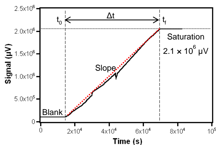
Figure 7. Experimental study of the saturation of the signal of detection. The concentration of formaldehyde used for this is 278 \mu\text{g m}^{-3} . The gas and liquid flow rates are 250 \text{ mL min}^{-1} and 17 \mu\text{L min}^{-1} , respectively. The volume of reagent is 5.79 mL and the microporous tube length is 10 cm. The black and dashed red lines correspond to the experimental values and the linear regression, respectively.
