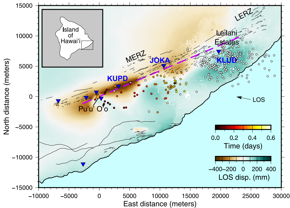
Fig. 1. May 2018 Dike propagation in the Middle East Rift Zone (MERZ) of the Kīlauea volcano. Circles are earthquake locations from the HVO catalog that occurred during the dike intrusion (circle colors indicate time relative to the 1st of May 2018). The assumed dike geometry is depicted with a purple dashed line. Background colors correspond to an unwrapped Sentinel-1 interferogram showing surface displacement in Line Of Sight (LOS) direction. Black lines shows mapped cracks and fissures and black triangles are vents from Trusdell et al. (2005). Seismic stations used in this study are blue triangles. The map on the upper left corner show the studied location. (For interpretation of the colors in the figure(s), the reader is referred to the web version of this article.)
