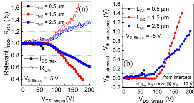
Fig. 2 (a) I_{DSS} , R_{ON} and (b) V_{TH} shift during off-state stress at V_{G,Stress} = -5 \text{ V} .
