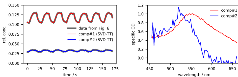
Figure S7. The two components of the rank-reduced SVD after transformation such that the concentration traces reproduce the concentration traces obtained in Figure 6 (main text). Left: concentration vectors ( \mathbf{C} = \mathbf{T}\mathbf{W}\mathbf{V}^T ), showing the modulation of gold NP concentration by DEP. Right: spectral vectors from the target-transformed SVD ( \mathbf{S} = \mathbf{U}\mathbf{T}^{-1} ), agreeing with the known spectra for Au40-LA and Au80-LA NPs.
