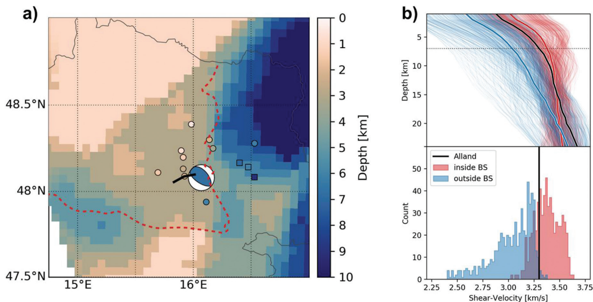
Figure 8: Regional context of the Alland earthquake. a) Alland earthquake near the edge of the Bohemian Spur (BS). Background image shows the first depth at which 2.9 km/s shear velocity is exceeded in the velocity model of Schippkus et al. (2018), which may be interpreted as the top of crystalline basement (see Schippkus et al., 2018 for more details). Crystalline basement depths, known from boreholes (marked as ○) or estimated from geological profiles (marked as □) from Wessely (2006). The beachball represents the Alland main shock, also coloured by depth. Red line marks the edge of the BS, redrawn from Wessely (2006). Black line marks the seismic profile C 8503 that crosses the borehole St. Corona 1 (see Fig. 9). b) Velocity model of Schippkus et al. (2018), classified by “inside” (red colour) and ‘outside’ (blue colour) the BS after Wessely (2006). Classification is based on the edge of the BS as drawn in Figures 1 and 8a. Top: velocity profiles, extracted at each grid node in a), extracted from Schippkus et al. (2018). Thick lines represent the mean velocity profiles inside (red) and outside (blue) the BS. The velocity profile at the location of the Alland sequence is drawn in black. The Alland profile (black) is similar to the mean velocity profile inside the BS (red). Bottom: Histogram of shear velocities at 7 km depth (source depth of Alland main shock, dotted line in top panel). Clear separation of faster and slower velocities by the classification with some overlap. The shear velocity found in 7 km depth near the Alland series (black line) appears more likely to be representative of the BS (red distribution).
