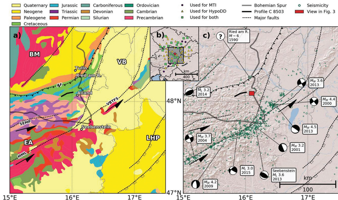
Figure 1: Map of the study region. a) Surface geology, extracted from the International Geological Map of Europe (IGME5000; Aschke, 2005). The thick grey line marks the edge of the “Bohemian Spur” after Wessely (2006). The thick black line near the centre marks the location of the seismic profile C 8503 (Fig. 9). Major faults (dashed lines) are redrawn after Peresson and Decker (1997). Labelled faults: Alpine Front (AF), SEMP fault, Mur-Mürz-Line (MML), Vienna Basin Transfer Fault System (VBTF). Labelled regions: Bohemian Massif (BM), Vienna Basin (VB), Eastern Alps (EA), and Little Hungarian Plain (LHP). b) Map of stations, classified by which parts of this study they are used in: moment tensor inversion (MTI), relocation with HypoDD, or both. c) Map of historical seismicity in the study region. Earthquakes are compiled from the Austrian Earthquake Catalogue (AEC, 2018) and the EMSC catalogue (Godey, 2006). Source mechanisms are extracted from the ISC Bulletin (Lentas et al., 2019) and are provided by ZAMG. The red rectangle marks the zoomed-in view shown in Figure 3 and location of the Alland earthquake sequence. Thin grey lines mark the Austrian borders and city border of Vienna.
