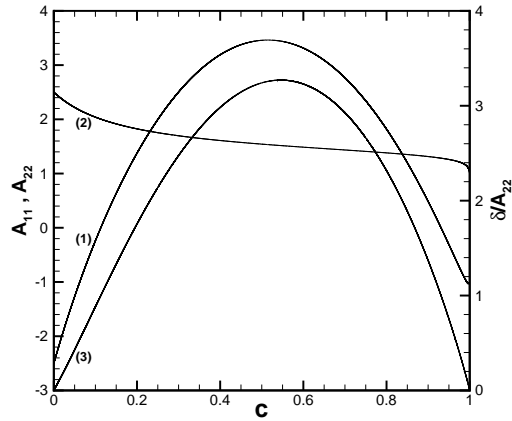
Fig. 2 Diagonal components of A, (1) A_{11} , (2) A_{22} ; (3) ratio \delta/A_{22} , vs. c , for q = 5
