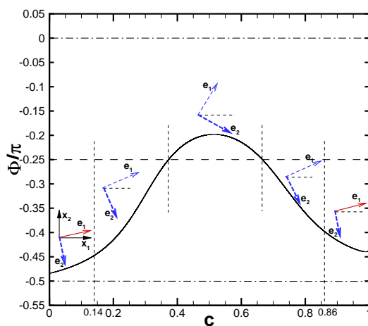
Fig. 7 Angle \Phi between x_1 and the direction of largest strain, e_2 , vs. c ; q = 1 ; a solid arrow indicates compressional strain, while a dashed arrow indicates extensional strain; direction of the largest strain is shown by a bold dashed arrow
