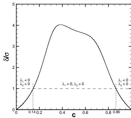
Fig. 6 Ratio \delta/\sigma and sign of strain eigenvalues vs. c ; q = 1
