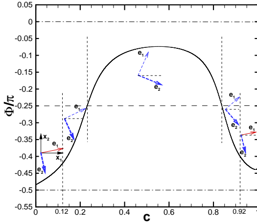
Fig. 4 Angle \Phi between x_1 and the direction of largest strain, e_2 , vs. c ; q = 5 ; a solid arrow indicates compressional strain, while a dashed arrow indicates extensional strain; direction of the largest strain is shown by a bold dashed arrow
