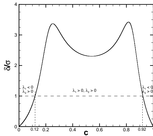
Fig. 3 Ratio \delta/\sigma and sign of strain eigenvalues vs. c ; q = 5
