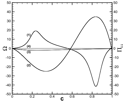
Fig. 5 Rotation rate of strain principal axes, \Omega , and components of pressure Hessian tensor, \Pi_{ij} , vs. c ; q = 5 ; (1) \Omega ; (2) \Pi_{11} ; (3) \Pi_{12} and \Pi_{21} ; (4) \Pi_{22}
