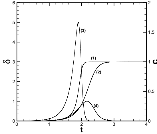
Fig. 1 Evolution of c and \delta ; (1) c(t) for q = 5 ; (2) for q = 1 ; (3) \delta(t) for q = 5 ; (4) for q = 1
