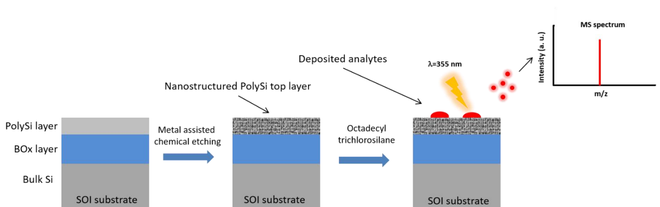
Figure 1: Schematic representation of the whole procedure to nanostructure Si based surfaces, their chemical modification and their use as SALDI surfaces for analytes MS detection.
