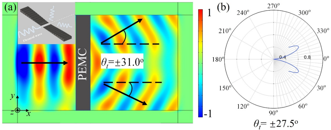
13 14 Fig. C1. (a) shows splitting the incident flexural wave by the PEMC. The model of the PEMC, which 15 consists of the two symmetrical supercells, is illustrated in the upper left corner. (b) illustrates the 16 polar directivity graph of the transmitted wave measured at two wavelengths away from the center 17 of the PEMC.
