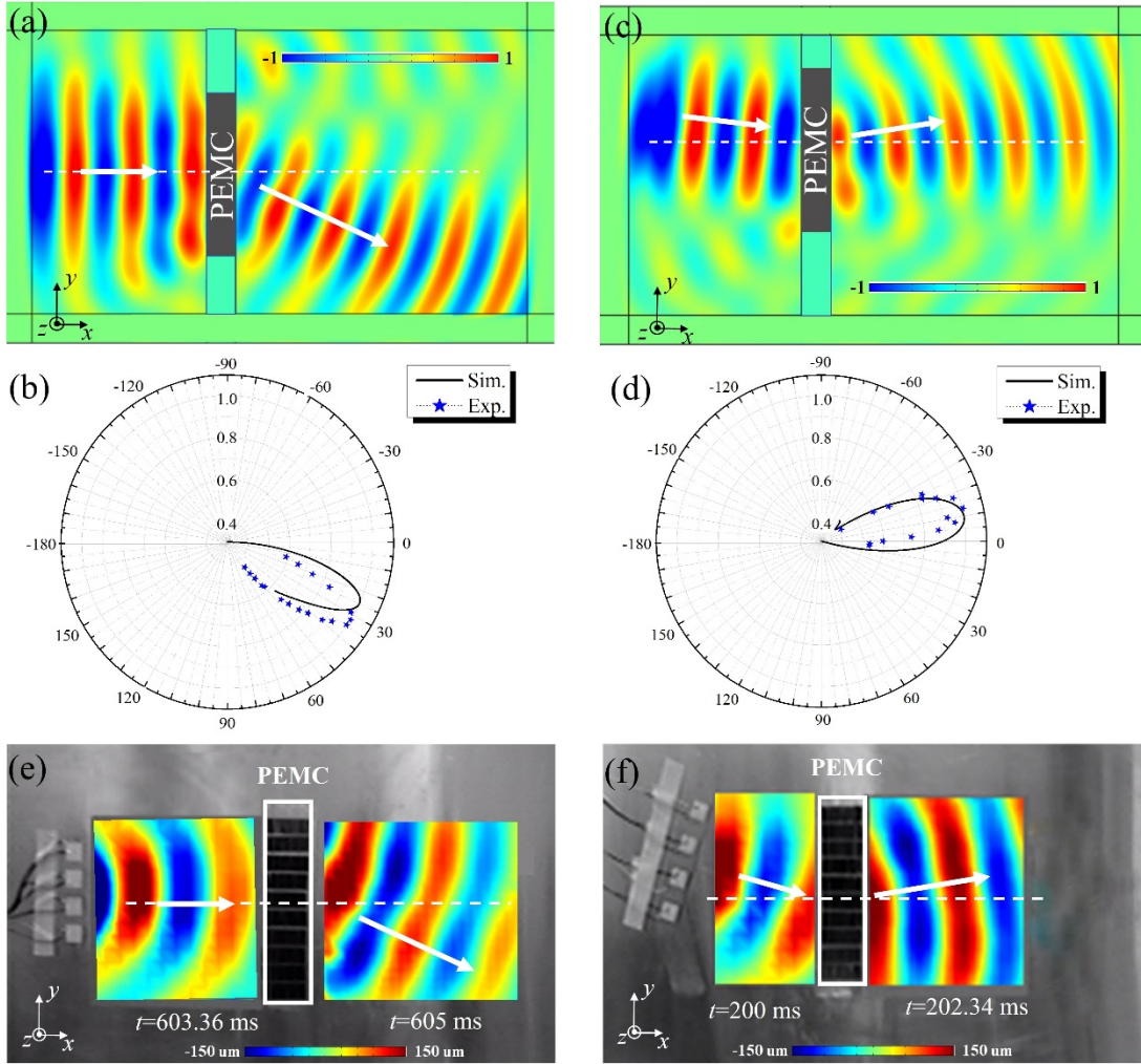
2 Fig. 6. The numerical simulation results for the vertically (a) and obliquely (c) incident waves across 3 the PEMC. Polar directivity graphs of the transmitted waves measured at two wavelengths away 4 from the center of the PEMCs are shown in (b) and (d), numerically and experimentally. The 5 experimental full wave fields including the incident field and the transmitted field at different time 6 points are shown in (e) and (f).
