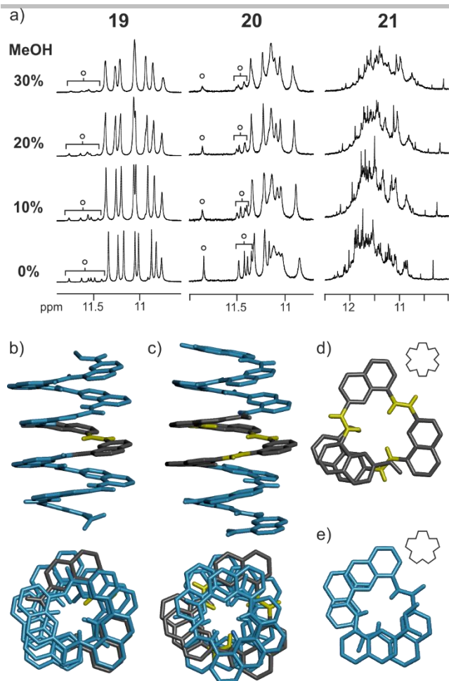
Figure 3. a) Part of the ^1\text{H} NMR spectra (300 MHz) of 19 , 20 and 21 in \text{CDCl}_3 containing different proportions of \text{CD}_3\text{OH} . Black circles in spectra of 19 and 20 , indicate the coexistence of a second conformer for these compounds. The spectra of 21 showed too many conformers to be identified. b, c) X-ray structures of 19 (b) and 20 (c). d, e) Comparison of the helix cross sections of 20 in its vinylic part (d) and its oligoamide part (e). Side chains and aromatic hydrogen atoms are removed for clarity; vinylene groups are highlighted in yellow. In d), the shape of an 18-crown-6 (top right) highlights the inner rim of the helix in the vinylic part. In e) the shape of an 15-crown-5 (top right) highlights the inner rim of the helix in the amide part
