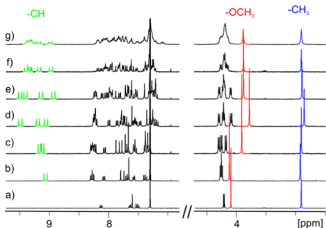
Figure 1. Part of the 1 H NMR spectra (300 MHz) of 1 and 6-11 at 298 K in CDCl 3 : a) 1 ; b) 6 ; c) 7 ; d) 8 ; e) 9 ; f) 10 ; g) 11 . Methyl ester, terminal aryl-methyl and vinyl proton signals are highlighted for all spectra in red, blue and green, respectively.
