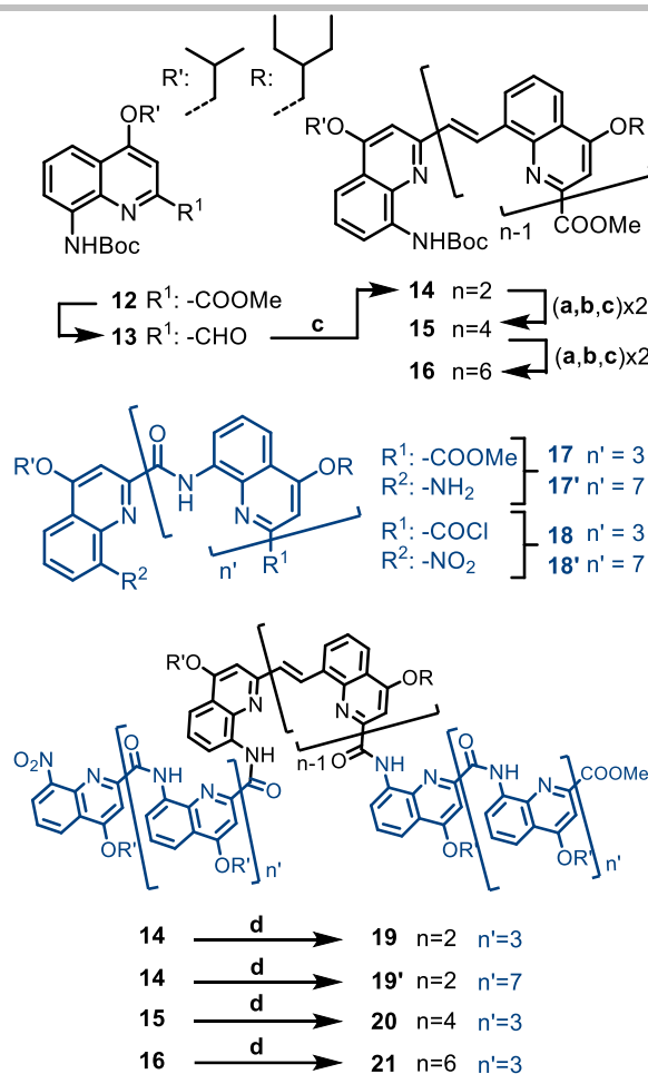
Scheme 3. Synthesis of quinoline oligoamide-oligovinylene hybrid foldamers. a: NaBH 4 , THF, 60°C; b: SIBX, THF 60°C; c: i) 5 , NaH, 15-crown-5, THF; ii) MeI, K 2 CO 3 , Acetone; d: i) NaOH, THF/MeOH, RT; ii) (COCl) 2 , CH 2 Cl 2 ; iii) 17 or 17' , i Pr 2 NEt, CH 2 Cl 2 ; iv) TFA, CHCl 3 ; v) 18 or 18' , i Pr 2 NEt, CH 2 Cl 2 .
