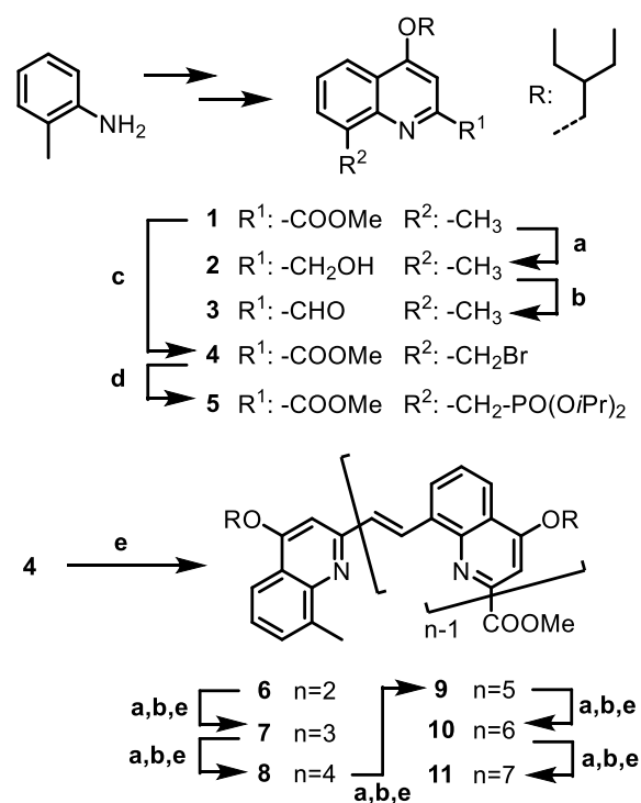
Scheme 2. Synthesis of quinolyne-vinylene oligomers. a: NaBH 4 , THF, 60°C; b: SIBX, THF 60°C; c: N-bromosuccinimide (NBS) S, CCl 4 , rfx; d: P(O i Pr) 3 ; e: i) 5, NaH, 15-crown-5, THF; ii) MeI, K 2 CO 3 , Acetone.
