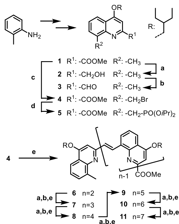
Scheme 2. Synthesis of quinolyne-vinylene oligomers. a: NaBH 4 , THF, 60°C; b: SIBX, THF 60°C; c: N-bromosuccinimide (NBS) S, CCl 4 , rfx; d: P(O i Pr) 3 ; e: i) 5, NaH, 15-crown-5, THF; ii) MeI, K 2 CO 3 , Acetone.
