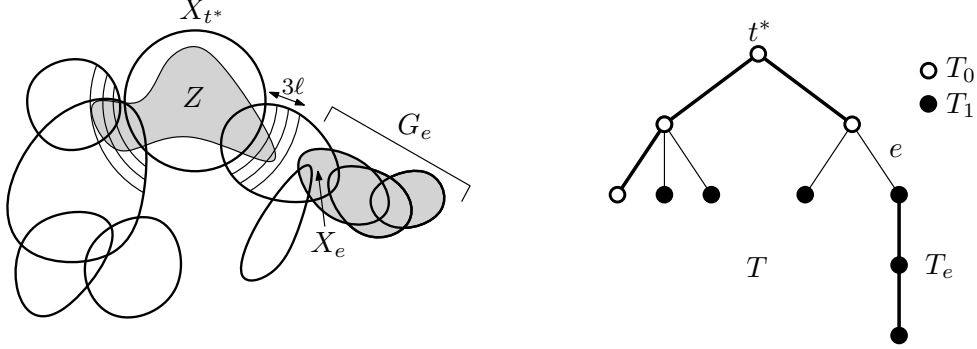
FIGURE 1. A snapshot of the setting of Lemma 3.2 and the notations used in the proof. Note that by Claim 3 we know that we can assume that Z = N_G^{\leq 3\ell}(X_{t^*}) , but we only include the original setting of this lemma in the picture.
