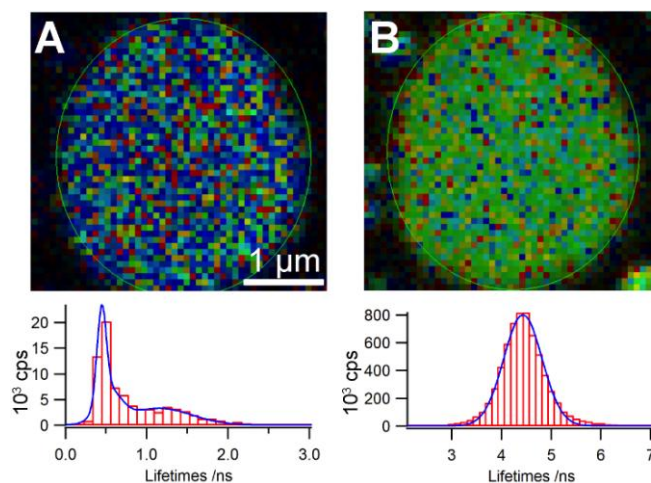
Fig. 3 Fluorescence lifetime imaging ( \lambda_{\text{ex}} = 375\text{nm} ) of a single blue-emitting aggregate deposited from solutions of m1 and p3 ( 100 : 1, 10^{-4} M in THF) collected at 400 – 450 nm (A) or 570 – 650 nm (B). In A, only the emission from m1 is observed and it exhibits a dual distribution of lifetimes in agreement with the existence of regions (blue patches) where no quenching by p3 is observed. The emission from p3 (B) shows a single lifetime distribution as expected for direct or sensitized excitation.
