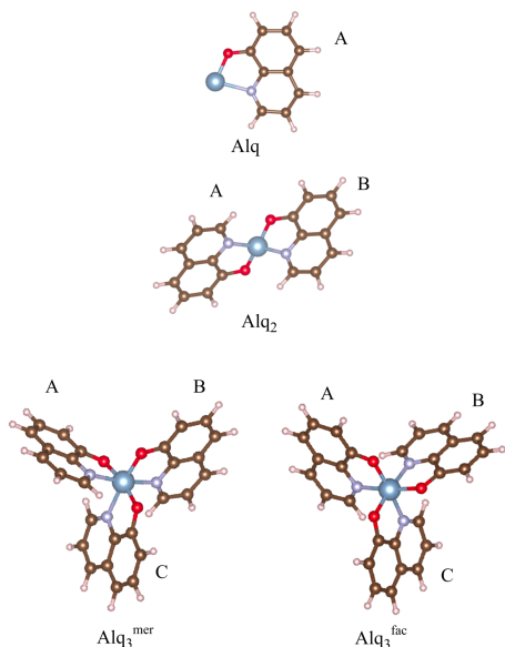
Fig. 3 Isolated Alq n ( n = 1, 2, 3 ) complexes. The Alq 3 species exists in meridional ( mer ) and facial ( fac ) isomers. A , B and C indicate the q molecules in the complex. Al atoms: big blue balls; O, N, C and H atoms: same colors as in Figure 2.
