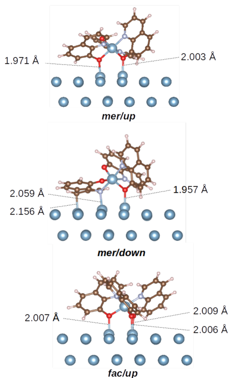
Fig. 4 Alq_3 complexes adsorbed on an Al(111) surface. Top: meridional up ( mer/up ). Middle: meridional down ( mer/down ) Bottom: facial up ( fac/up ); for practical purposes, only two layers of the Al(111) slab are shown.
