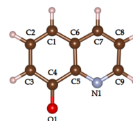
Fig. 2 The q molecule. O atom: red ball; N atom: blue ball; C atoms: brown balls; H atoms: white balls.
