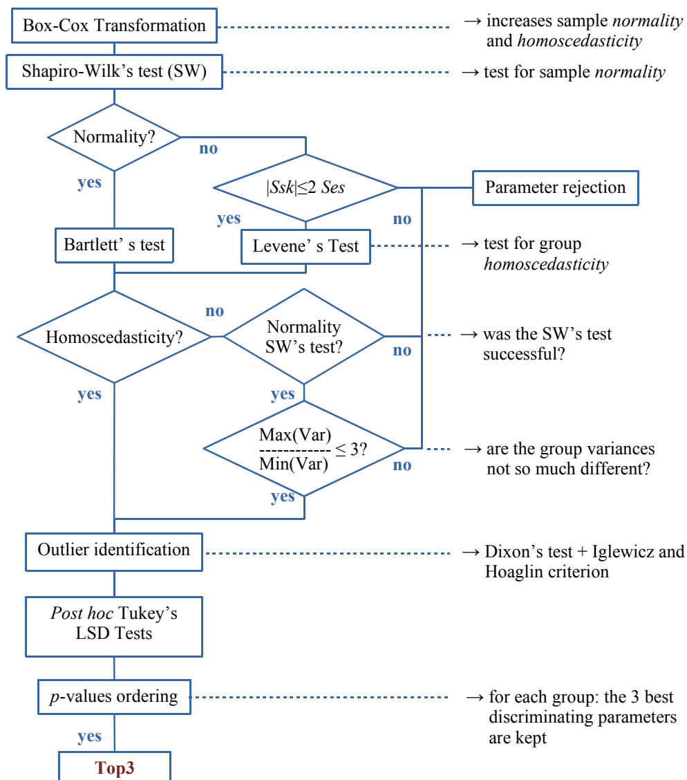
Figure 2. Synopsis of the procedure with all of the parameters as the input, and the three most discriminative ones as a result (Top3).
