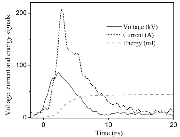
Fig. 1. Voltage, current and energy signals for a typical 85 kV peak voltage pulse.
