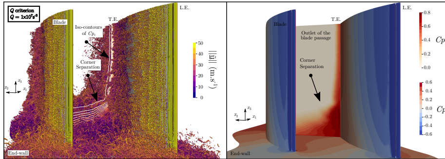
Figure 5: Visualisation of the LES flow field. Left: instantaneous Q criterion iso-surface ( Q = 1 \times 10^7 \text{ s}^{-2} ). Right: Mean pressure coefficient on the blade and the end-wall, and mean total pressure coefficient at the outlet of the blade passage. The same scale and colourmap are used for C_{p_t} in both figures.
