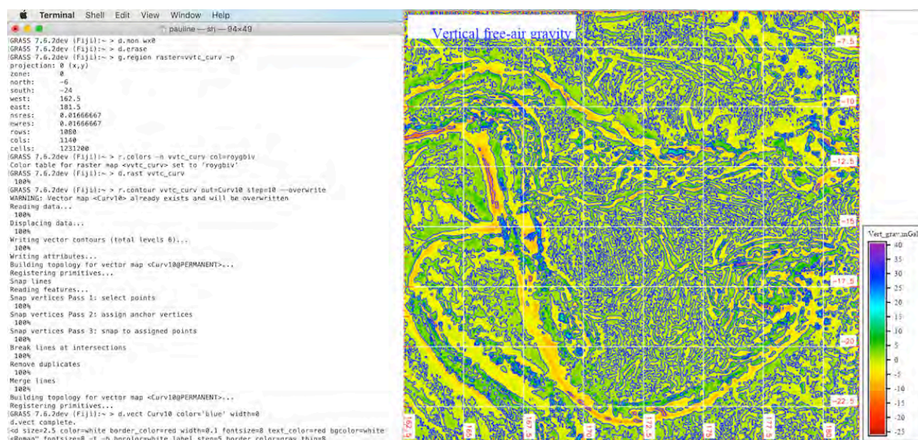
Fig. 5. Vertical marine free-air gravity anomaly, Fiji region, south Pacific Ocean. Visualization of the grid (.grd) file extracted as a subset of img file (vvtc_curv.grd) in geographic format based on CryoSat-2 measurements. Left: GRASS GIS shell console. Right: GRASS GIS map output. Source: author.
