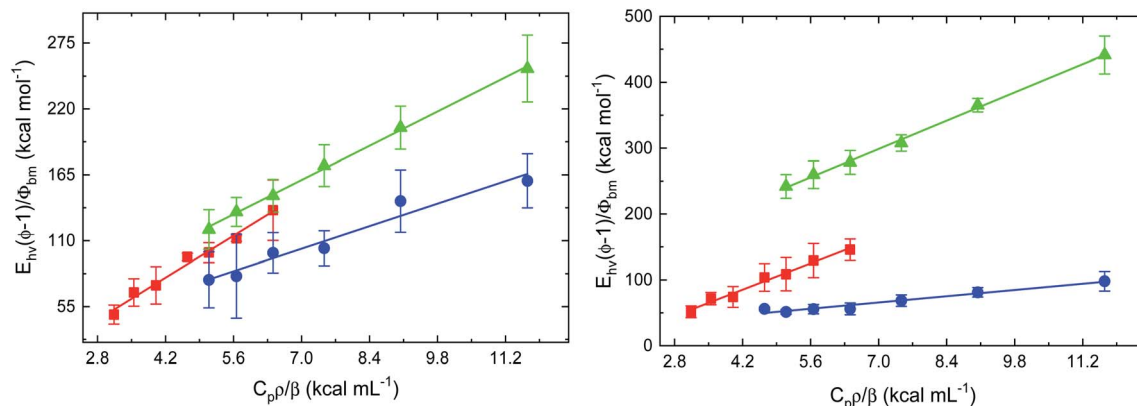
Fig. 3 Plots of E_{nv}(\phi - 1)/\Phi_{bm} vs. C_p\rho/\beta for photo-dissociation of CO from CO-FHP (left) and CO-HMP Sa (right) in the absence of drug compounds (red), with 8.5 \mu M ketoconazole (blue), and with 408 \mu M miconazole (light green).
