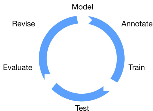
Figure 7: MATTER workflow
