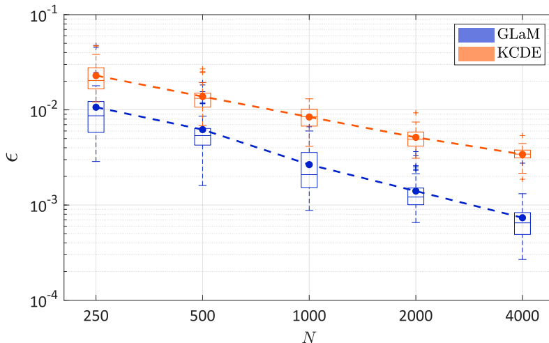
Figure 21: SIR model, mean value estimations – Comparison of the convergence between GLaMs and KCDEs in terms of the normalized mean-squared error as a function of the size of the experimental design. The dashed line denotes the average value over 50 repetitions of the full analysis.
