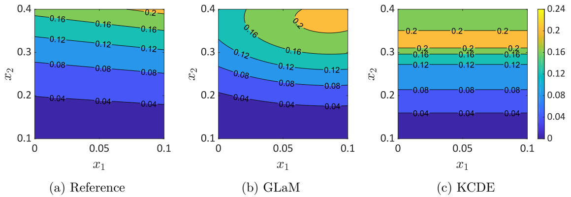
Figure 4: Example 1 – Comparisons of the variance function estimation, N = 500 .
