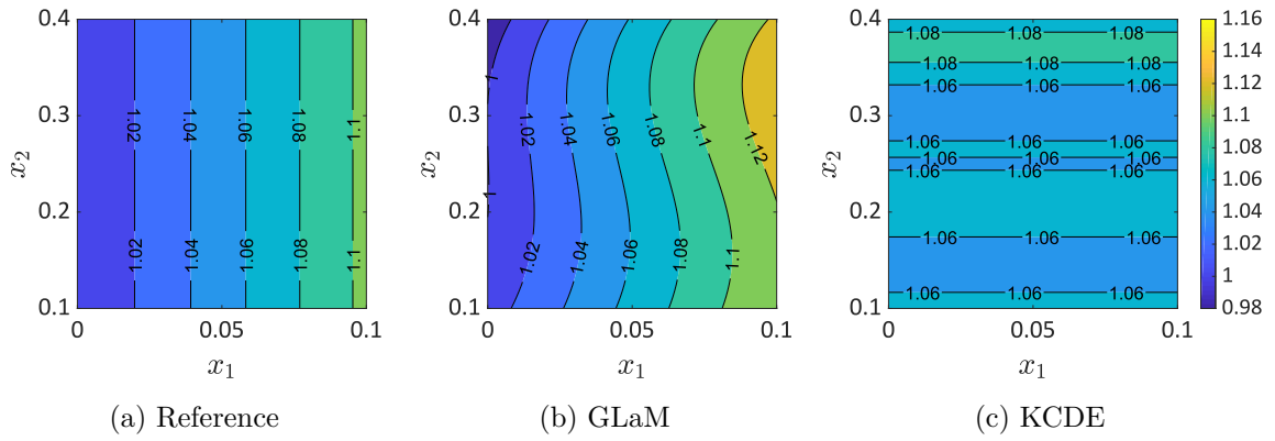
Figure 3: Example 1 – Comparisons of the mean function estimation, N = 500 .
