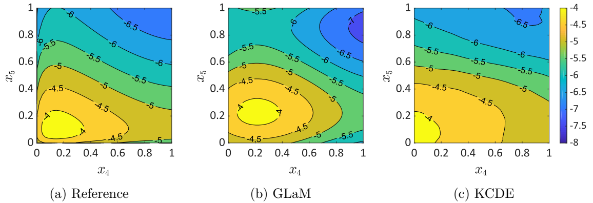
Figure 7: Example 2 – Comparisons of the mean function estimation in the plan x_4 - x_5 with all the other input fixed at their expected value. The surrogate models are fitted to an ED with N = 1,000 .
