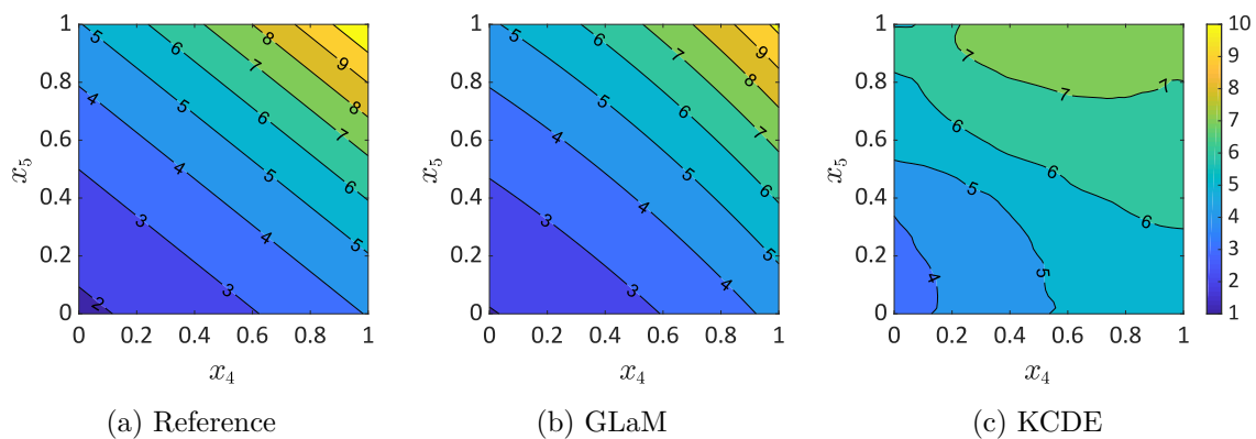
Figure 8: Example 2 – Comparisons of the variance function estimation in the plan x_4 - x_5 with all the other input fixed at their expected value. The surrogate models are fitted to an ED with N = 1,000 .
