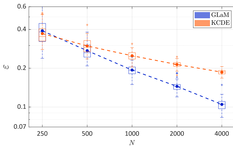
Figure 9: Example 2 – Comparison of the convergence between GLaMs and KCDEs in terms of the normalized Wasserstein distance as a function of the size of the experimental design. The dashed lines denote the average value over 50 repetitions of the full analysis.
