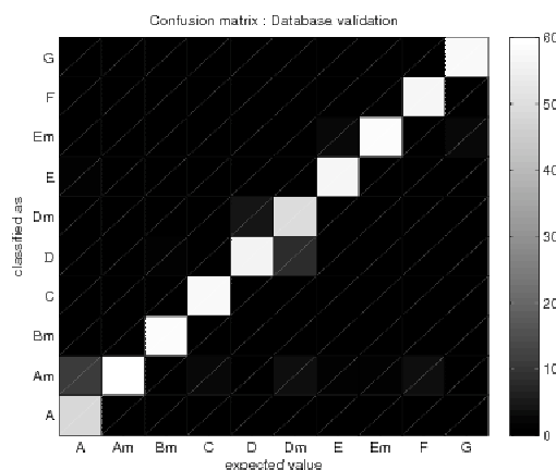
Figure 4. Confusion matrix for a network trained with a mixed learning set of 1400 samples (140 chords per class). The test set contains 600 samples (60 per class). The total error rate is 6.5%.
