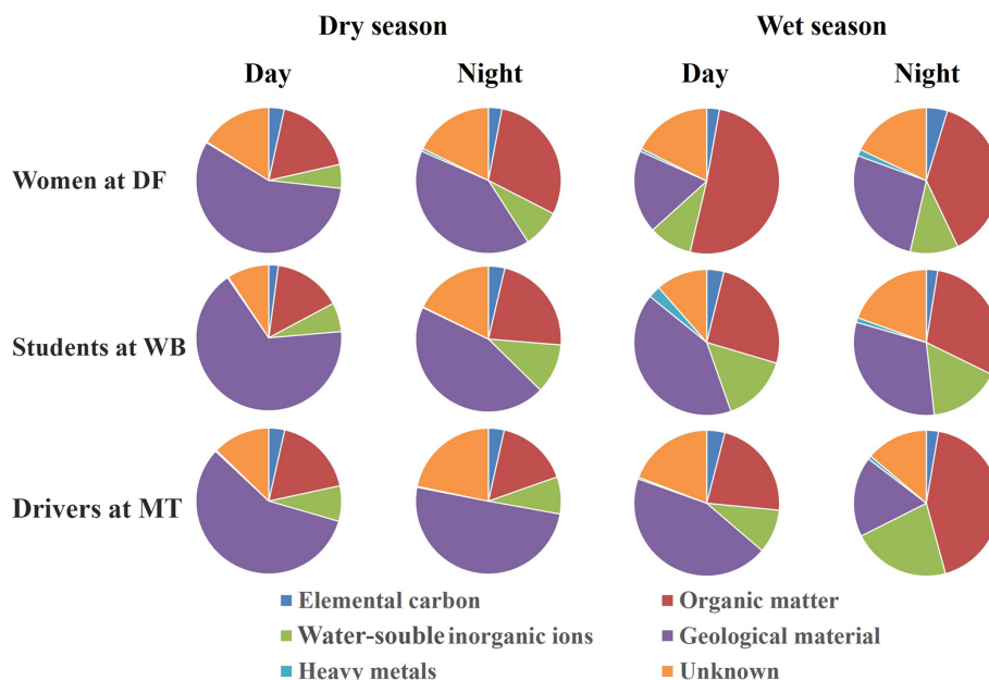
Figure 5. Personal exposure to PM 2.5 mass concentration closures for women at DF, students at WB and drivers at MT in different sampling seasons.
