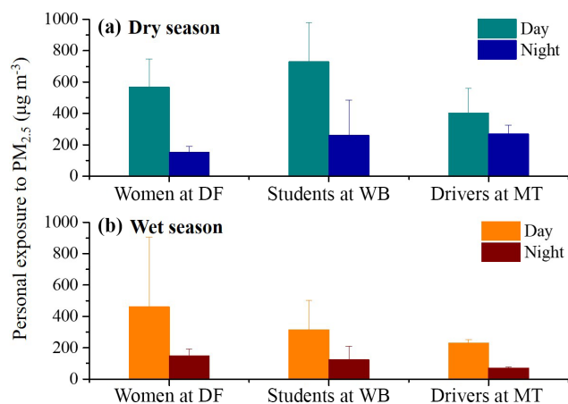
Figure 3. Personal exposure to PM 2.5 mass concentrations of women at DF, students at WB and drivers at MT in the dry season (January) and wet season (July) of 2016 in the sWA area.
