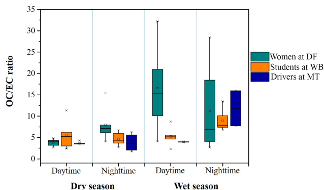
Figure 4. Variations of OC/EC ratios in personal exposure to PM 2.5 samples for women at DF, students at WB and drivers at MT. (The box plots indicate the average concentration and the min, 1st, 25th, 50th, 75th, 99th and max percentiles).
