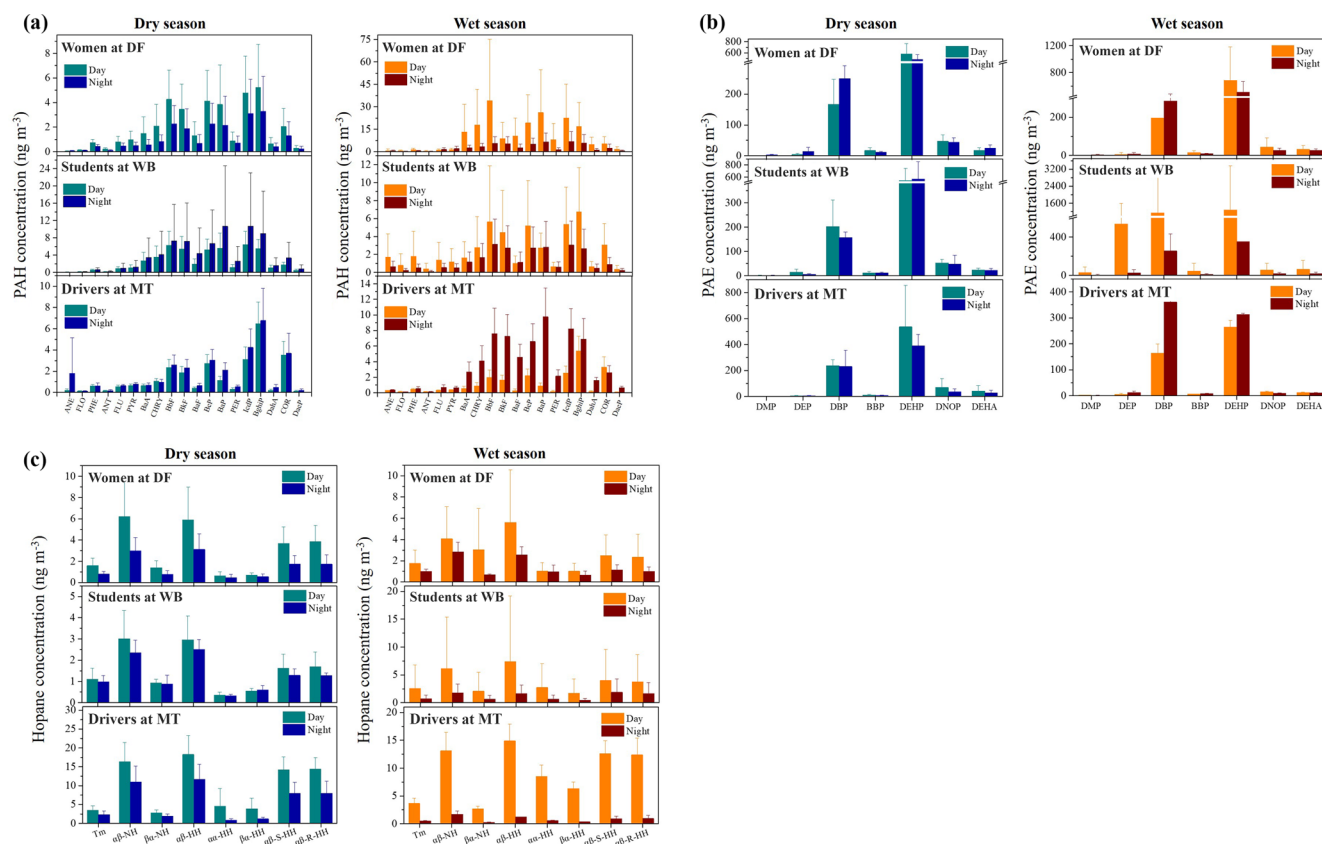
Figure 6. Distributions of (a) PAHs, (b) PAEs and (c) hopanes in PM 2.5 personal exposure samples for women at DF, students at WB and drivers at MT in dry and wet seasons of 2016.
