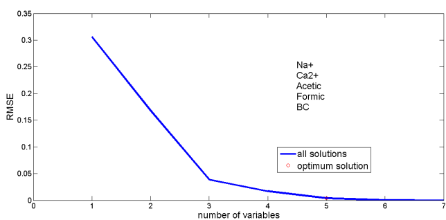
Figure 16: Ionic MLR modelled in the instance where OC was dependent variable and all other ions independent.
