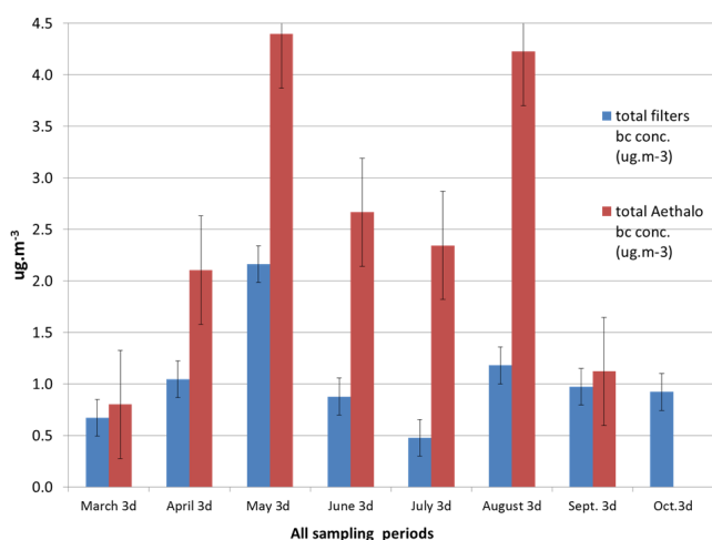
Figure 8: Comparison of filter sampling BC with aethalometer BC trends over the same three days in each sampled month. Note that the aethalometer values were adjusted 30% lower to account for scattering and other reasons as per Hansen et al. (1984). Impactor concentrations were unchanged (mean ± SEM).
