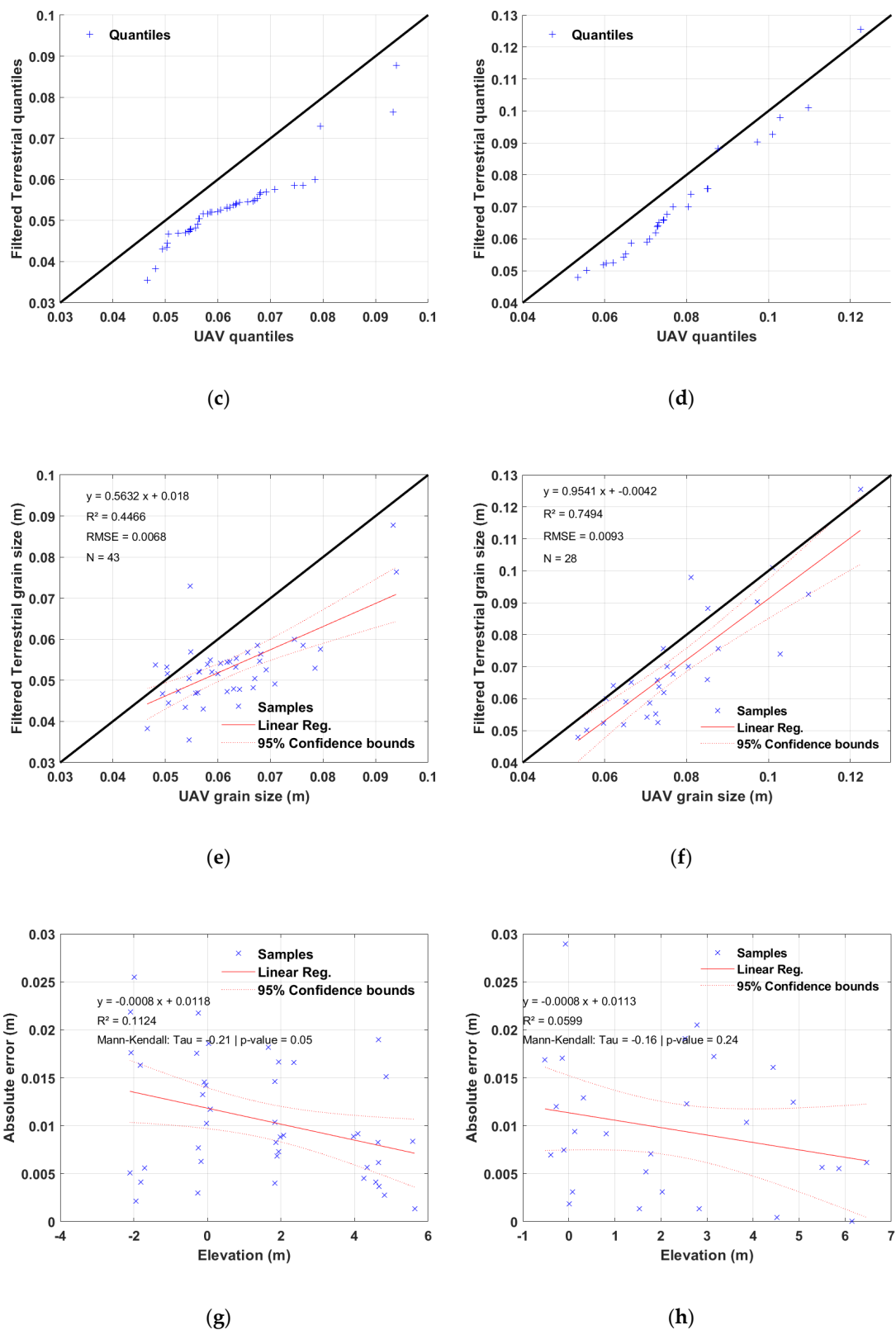
Figure 11. Clast size mapping validation results. (a,b): Comparison of the average grain size as measured on the terrestrial samples (blue “x” symbols), the filtered terrestrial samples (red “o” symbols) and by the UAV samples (black “+” symbols at (a) Etretat and (b) Hautot-sur-Mer. Colored envelopes present the standard deviation intervals. Compared mean values of the UAV and filtered terrestrial distributions at (c) Etretat and (d) Hautot-sur-Mer. Quantile–Quantile diagrams comparing the UAV and filtered terrestrial distributions at (e) Etretat and (f) Hautot-sur-Mer. Absolute error on the pebble size measurements as a function of the elevation at (g) Etretat and (h) Hautot-sur-Mer.
