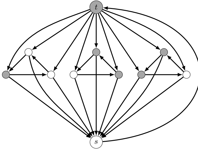
Figure 2: A strongly connected twin-free and quasi-twin-free digraph of order n with location-domination number \frac{2(n-2)}{3} , with a locating-dominating set in grey.
