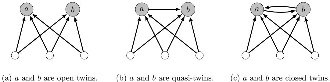
Figure 1: Examples of twin vertices.
