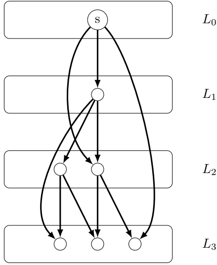
Figure 4: The levels in the proof of Theorem 16.
