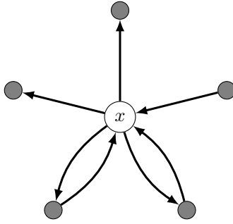
Figure 3: A directed star, with a minimum locating-dominating set in grey.
