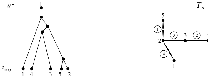
FIGURE 5. In the figure on the left, an example of a pseudo-trajectory with N_k = 5 . The associate graph T_{\prec} is depicted on the right. For instance there holds G_2 = \{(2, 5)(3, 4)\} and (q_3, \bar{q}_3) = (2, 3) .
