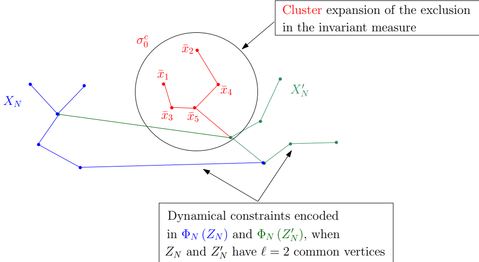
FIGURE 4. Cluster expansion of the exclusion when Z_N and Z'_N have \ell common elements. The constraints imposed by \Phi_N(Z_N) and \Phi_N(Z'_N) are no longer independent, and the 2(N-1) dynamical constraints will be replaced by 2N-\ell-1 “independent” dynamical constraints (by extracting from the blue and green graphs a minimally connected graph). In this case X_{2N-\ell} is considered as one vertex for the exclusion expansion.
