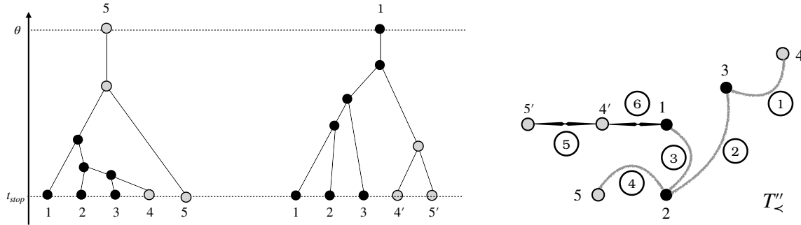
FIGURE 6. In the figure on the left, an example of 2 pseudo-trajectories sharing \ell = 3 particles with N_k = 5 . The graph T_{\prec} associated with the left pseudo-trajectory starting from Z_5 is depicted by the bended grey edges ordered according to the encounter times. The complete tree T''_{\prec} is built starting from T_{\prec} to which two additional straight edges (numbered 5 and 6) have been added to connect 4' and 5'.
