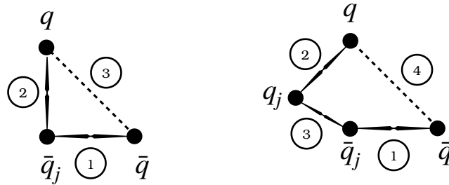
FIGURE 12. Graphs associated to the pseudo-trajectories in Figure 11. Non clustering encounters are represented by dashed lines.
