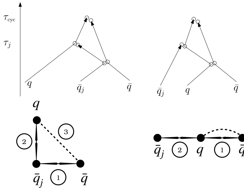
FIGURE 9. Two simple situations corresponding to Case 1b. The non clustering encounter between (q, \bar{q}) is triggered by a previous deflection between q = q_j and \bar{q}_j which is not equal to \bar{q} . The parameter \hat{x}_j has to be tuned so that the encounter between q, \bar{q}_j leads as well to the recollision. The corresponding graphs with a cycle are depicted below.
