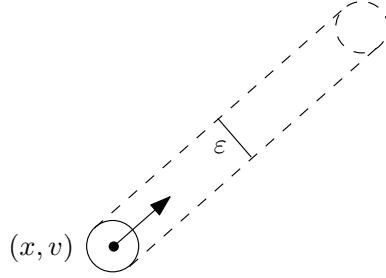
FIGURE 2. The collision cylinder of diameter \varepsilon has volume proportional to \varepsilon^{d-1}|v|\tau , where \tau is the time of free flight.
