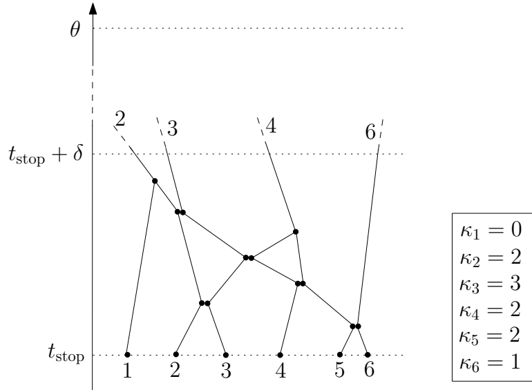
FIGURE 7. Example of pseudo-trajectory with recollisions in the time interval (t_{\text{stop}}, t_{\text{stop}} + \delta) . The associated forward flow is determined thanks to the recollision indices at time t_{\text{stop}} , listed on the right.
