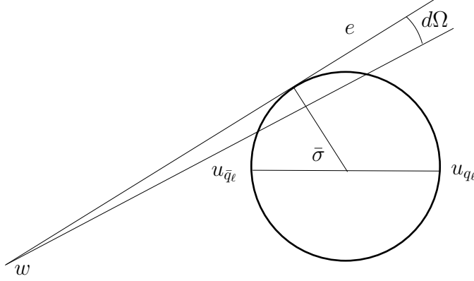
FIGURE 13. The geometry leading to the degeneracy at \sigma_\ell = \bar{\sigma} of the singular integral (B.13) is depicted.
