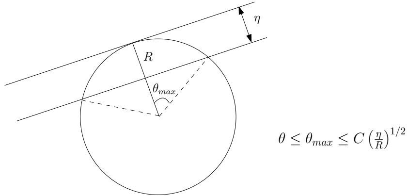
FIGURE 10. Intersection of a cylinder and a sphere. The maximal solid angle is obtained in the case when the cylinder is tangent to the sphere. It is always less than C_d \min(1, (\eta/R)^{(d-1)/2}) .
