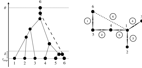
FIGURE 8. In the pseudo-trajectory (with N_k = 6 ) represented on the left figure, a recollision occurs between 5, 6 in the time interval [t_{\text{stop}}, t_{\text{stop}} + \delta] . Therefore the graph encoding all encounters is not minimal, and it has at least one cycle (or multiple edge). The time ordering of the clustering and non clustering encounters is represented by the circled numbers and the edges are added dynamically following the forward dynamics, i.e. starting from t_{\text{stop}} . As a consequence, the recollision between 5, 6 in the backward pseudo-dynamics becomes the first clustering encounter in the forward dynamics and the non clustering encounter is identified with the dashed edge (1, 6) occurring close to time \theta .
