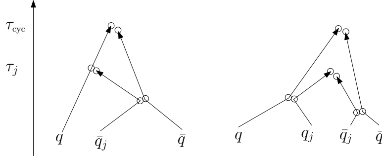
FIGURE 11. Two simple situations corresponding to Case 2. In the picture on the left, only three particles are involved and \bar{q}_j is annihilated in the encounter with q at time \tau_j ( j \geq 2 ). The picture on the right depicts another possible situation, where 4 particles are involved as q, \bar{q} are both different from q_j, \bar{q}_j ( j \geq 3 ).
