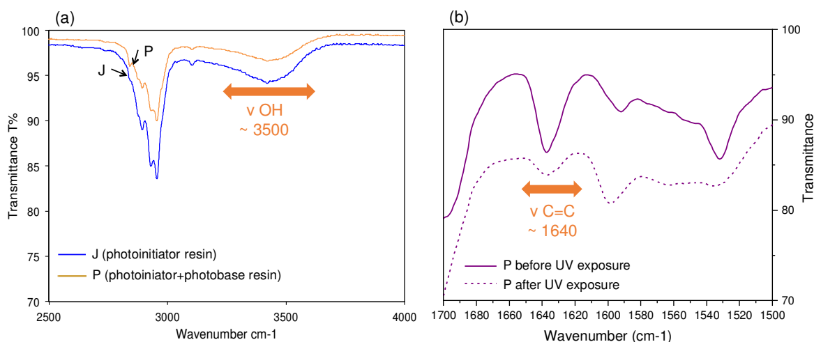
Fig. 7 (a) IR spectra on films of the photobase resin (resin P) and the photoinitiator resin (resin J) as reference, focusing on the OH elongation band at 3500\text{ cm}^{-1} (b) IR spectra on films of the photobase resin (resin P) before and after UV exposure, focusing on the C=C elongation band at 1640\text{ cm}^{-1}
