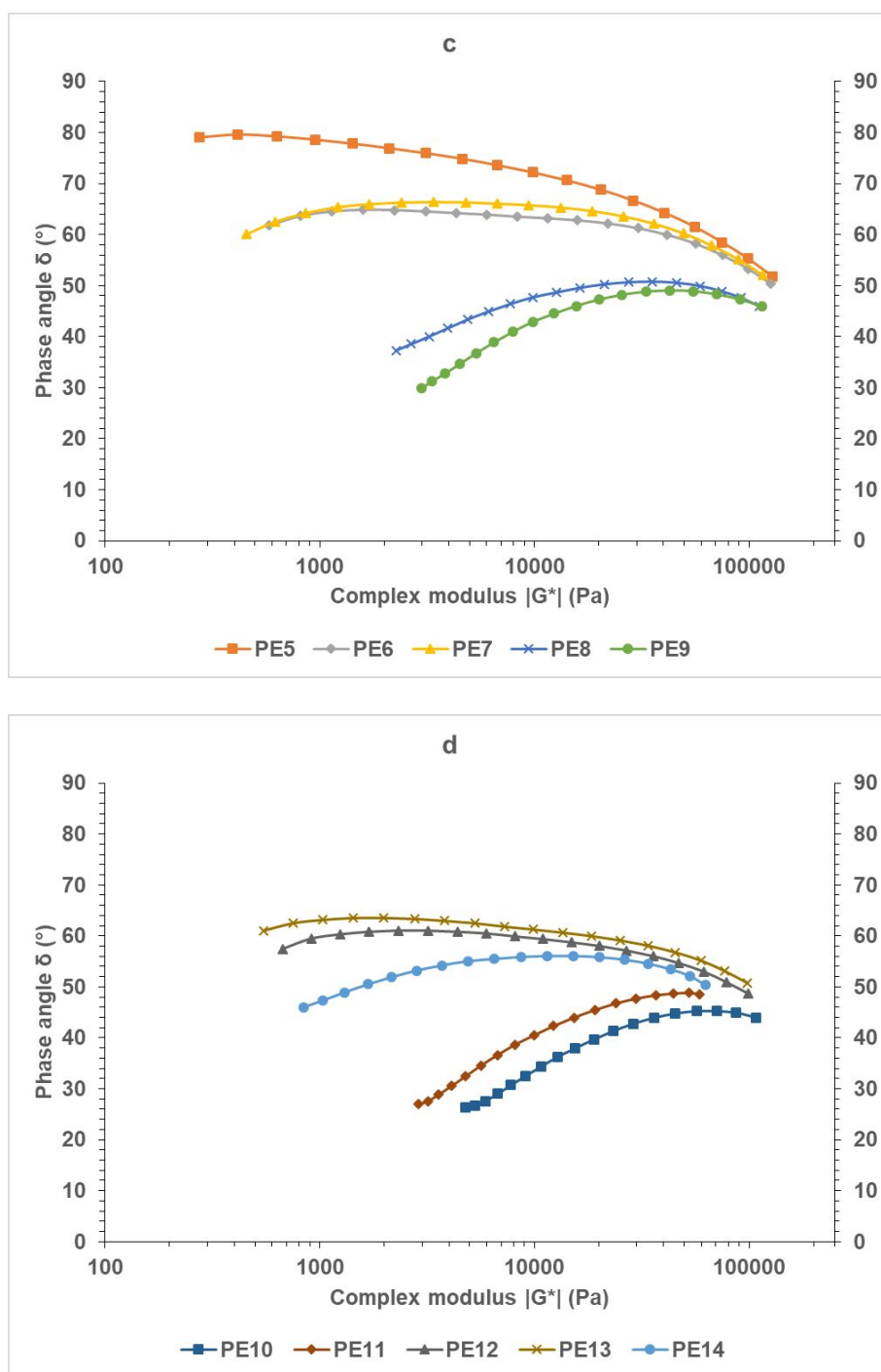
Figure 3. Rheological properties of the PEs obtained with supp-Zr-1/TIBAL/Al-1 systems: (a, b) complex viscosity ( |\eta^*| ) vs angular frequency ( \omega ) plot, (c, d) van Gorp-Palmen plot. Shear strain ( \gamma ) 10%, angular frequencies ( \omega ) from 0.1 to 250 \text{rad}\cdot\text{s}^{-1} , T = 190\text{ }^\circ\text{C} .
