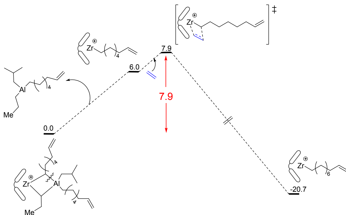
Scheme 7. The profile for an insertion of ethylene monomer to [\text{rac}\{-\text{EBTHI}\}\text{Zr}-(\text{oct-7-en-1-yl})]^+ formed via the cleavage of the Al–alkenyl bond and subsequent oct-7-en-1-yl group transfer. Note, the adduct-less interaction of the monomer suggests a more rapid insertion of ethylene.
