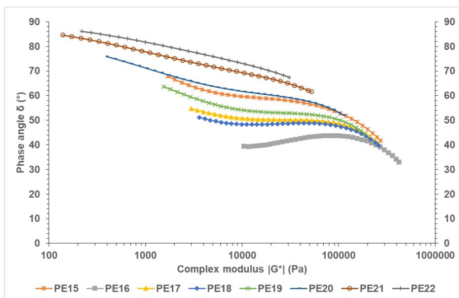
Figure 4. Van Gurp-Palmen plot of the PEs obtained with supp-rac -{EBTHI}ZrCl 2 /TIBAL/ AI-1 system with different amounts of H 2 . Shear strain ( \gamma ) 10%, angular frequencies ( \omega ) from 0.1 to 250 rad·s -1 , T = 190^\circ\text{C} .
